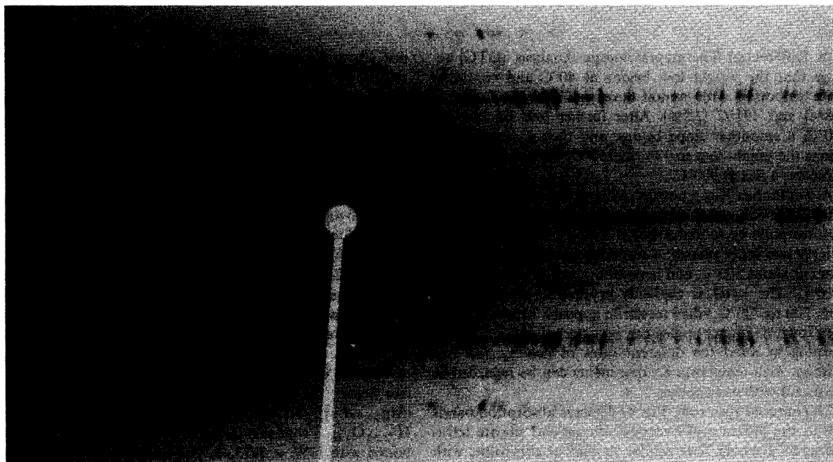
Fig. 4. b -rotation photograph of carlosturanite (Ni-filtered \text{CuK}\alpha radiation). The 5.2 Å layer lines of intergrown chrysotile are shown by arrows.
