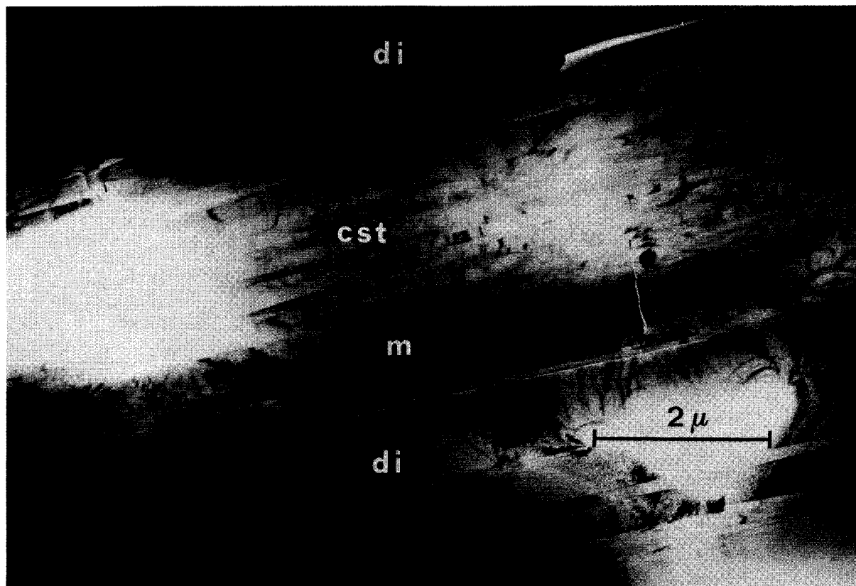
Fig. 2. TEM image of parallel intergrowth of diopside (di) and carlosturanite (cst). The opaque inclusion (m) is chromian magnetite.
