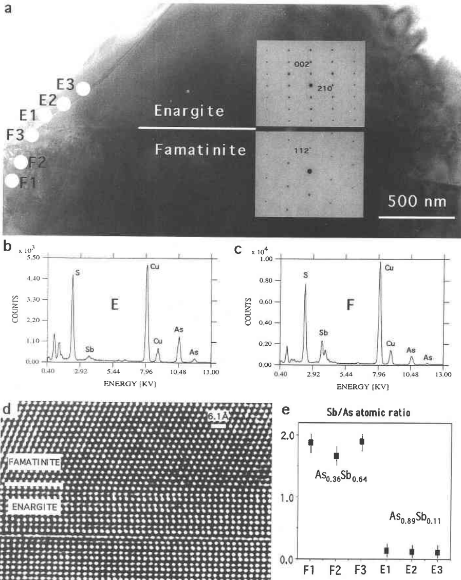
FIGURE 2. (a) Low-magnification image of a coherent intergrowth of enargite and famatinite with corresponding SAED patterns; typical EDS spectra obtained from (b) enargite and (c) famatinite; (d) high-resolution image of the interface; and (e) Sb/As atomic ratios obtained from the areas marked by white spots in (a).
