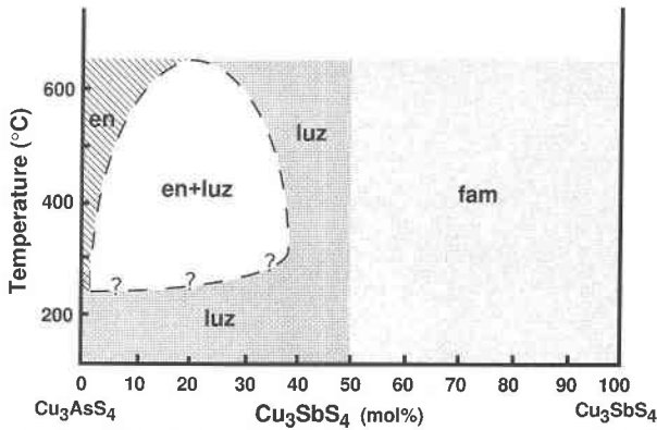
FIGURE 1. Temperature-composition diagram of the \text{Cu}_3\text{AsS}_4 - \text{Cu}_3\text{SbS}_4 join (en = enargite; luz = luzonite; fam = famatinite). After Barton and Skinner (1967) and Feiss (1974), and modified on the basis of data by Maske and Skinner (1971) and Sugaki et al. (1982).
