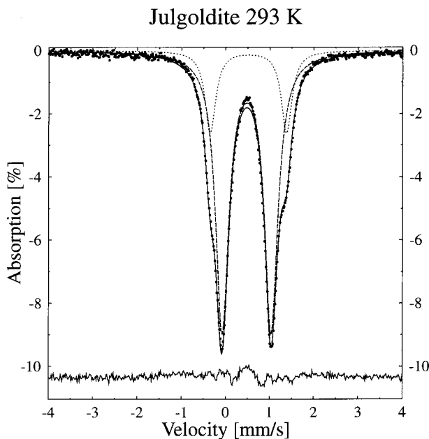
FIGURE 1. 57 Fe Mössbauer spectrum of julgoldite (sample JULG-A) showing a two doublet fit. The fit parameters are listed in Table 2.
