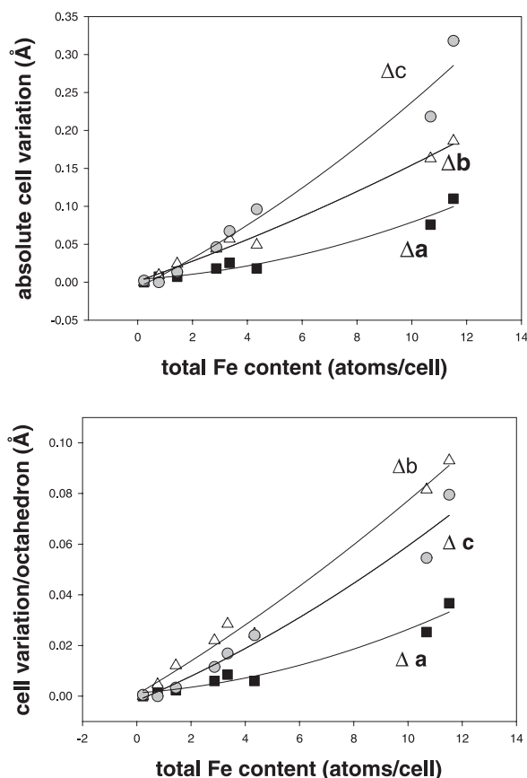
FIGURE 4. (a) Variation of the unit-cell parameters as a function of the total Fe content in pumpellyite and julgoldite minerals. (b) Variation in the unit-cell parameters as a function of the total Fe content normalized against the number of octahedral sites in each crystallographic direction. Sources of data are as in Figure 3.
