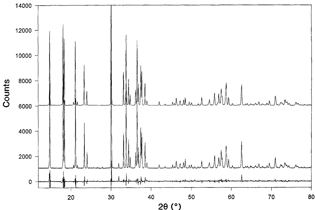
FIG. 1. The observed (middle), calculated (top) and difference (bottom) X-ray diffraction patterns for olivenite refined in the space group P2_1/n ; the observed and calculated patterns have had 1000 and 6000 counts added to each data point for clarity.
