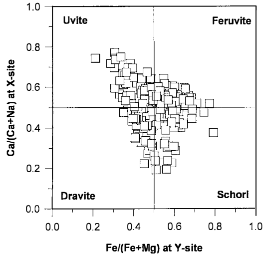
FIG. 3. Plot of \text{Ca}/(\text{Ca} + \text{Na}) at the X site versus \text{Fe}/(\text{Fe} + \text{Mg}) at the Y site in tourmaline from the exocontact of the lepidolite pegmatite. Quadrants are labeled according to the dominant tourmaline end-members.
