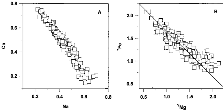
FIG. 4. A. Ca versus Na (apfu). B. 7 Fe versus 7 Mg (apfu) for tourmaline in the exocontact of the lepidolite pegmatites. The line represents a slope of -1.
