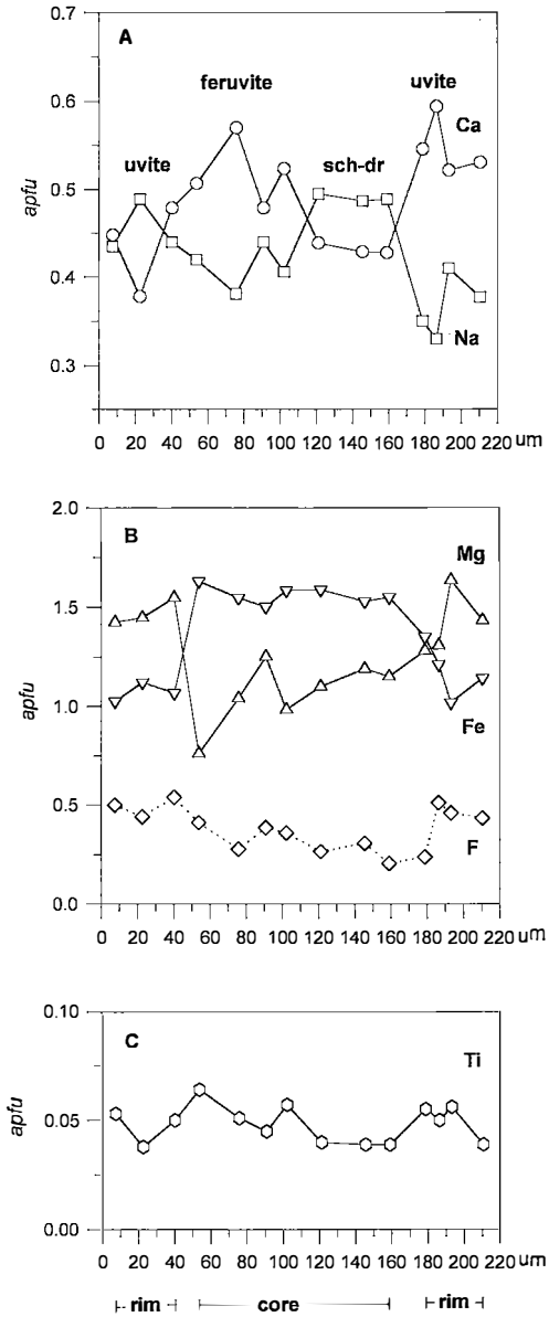
FIG. 2. Compositional variations for the traverse along the length of the 0.22 \times 0.05 mm grain shown in Figure 1; sch-dr: schorl – dravite.
