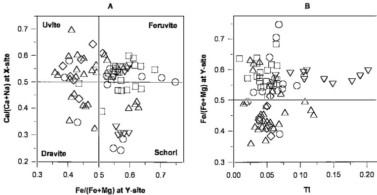
FIG. 5. Color versus composition of tourmaline from the exocontacts of the lepidolite pegmatites. A. Ca/(Ca + Na) at the X site versus Fe/(Fe + Mg) at the Y site. B. Fe/(Fe + Mg) versus Ti (apfu). Circles represent green tourmaline, squares represent dark blue tourmaline, triangles represent blue tourmaline, diamonds represent pale blue tourmaline, and inverted triangles represent brown tourmaline.
