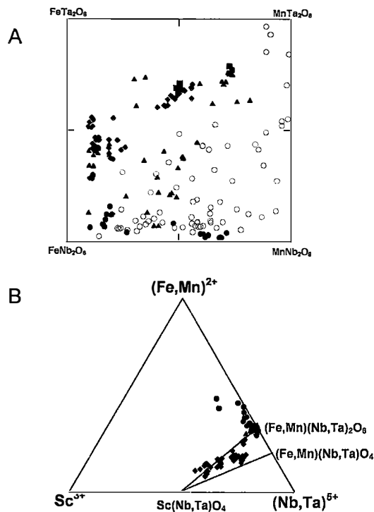
FIG. 1. Plot of Sc-bearing columbite and ixiolite in (A) columbite quadrilateral and (B) the Sc – (Fe, Mn) – (Nb, Ta) diagram. Open circles: scandian columbite, diamonds: scandian ixiolite, squares: stannian ixiolite, triangles: titanite ixiolite, dots: wolframian ixiolite. Black field in B represents data for columbite and stannian and titanite ixiolites.
