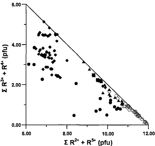
FIG. 2. Relationship between \Sigma R^{3+}R^{4+} and \Sigma R^{2+}R^{5+} cations (atoms pfu ). Symbols as in Figure 1.
