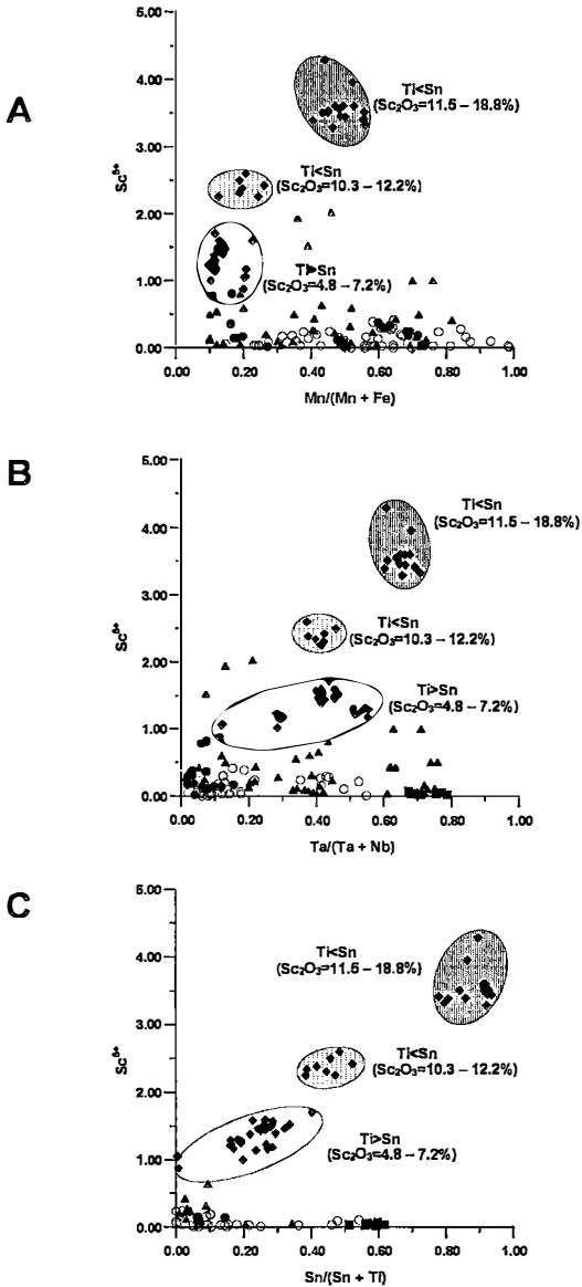
FIG. 4. Correlation of amounts of Sc with relative enrichment in (A) Mn, (B) Ta and (C) Sn. Symbols as in Figure 1.
