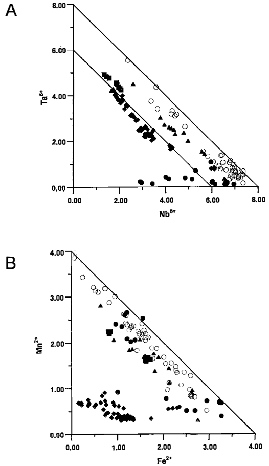
FIG. 3. Variation diagrams. (A) Nb versus Ta; (B) Fe versus Mn (atoms pfu ). Symbols as in Figure 1. Upper and lower boundaries represent trends of ideal \text{AB}_2\text{O}_6 and \text{ABO}_3 stoichiometries, respectively.
