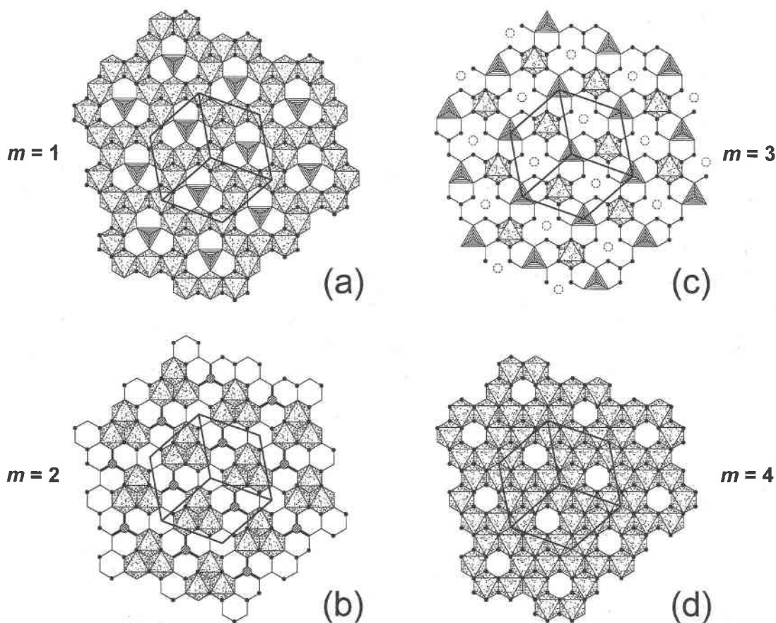
FIG. 2. The polyhedral layers for m = 1 to m = 4 in arakiite and hematolite: (a) m = 1 ; (b) m = 2 ; (c) m = 3 ; (d) m = 4 ; MO_6 octahedra: random dot-shading; AsO_4 tetrahedra: line-shading; As^{3+} cations: large diagonal-line-shaded circles; As^{3+}-O bonds: thick lines; small shaded circles: (OH) groups; broken circles: anion vacancies.
