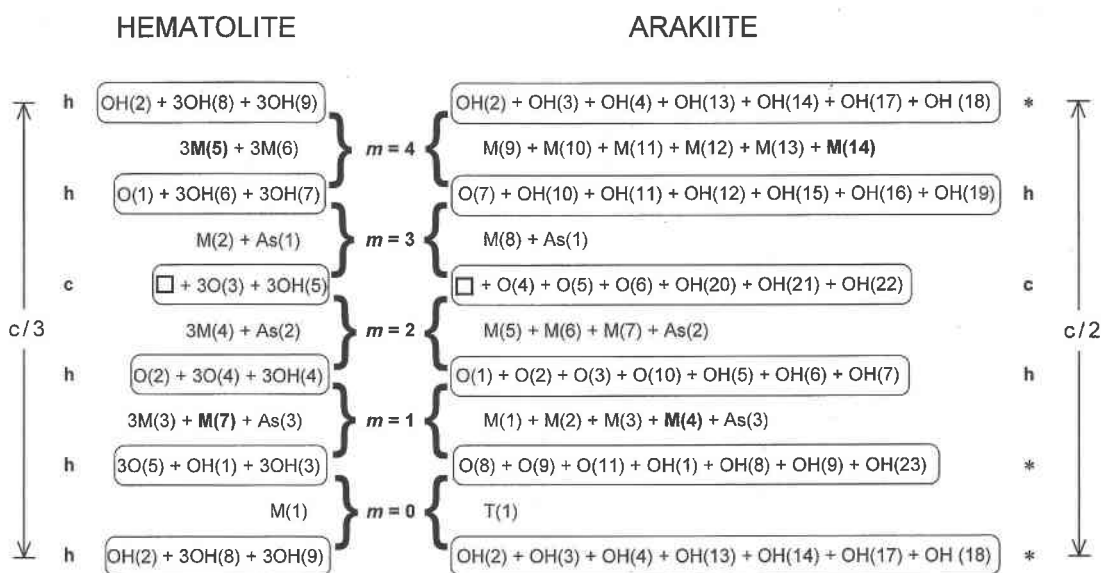
FIG. 3. The sheet-stacking sequences in hematolite (left) and arakiite (right). The various anion layers are shown in round-cornered boxes, together with the type of anion packing ( c : cubic close-packed, h : hexagonal close-packed, *: non-close-packed) at the left and right margins of the figure. The cations of the sheets are shown intercalated between the anion layers with the sheet numbering ( m = 0 to m = 4 ) shown in heavy symbols at the center of the diagram. The cation sites denoted in bold contain octahedrally coordinated trivalent cations ( \text{Fe}^{3+} and Al); coefficients denote number of sites pfu .
