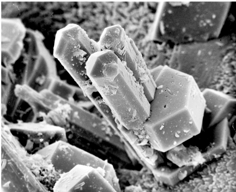
FIG. 1. Slender prismatic crystals of henrymeyerite intergrown with stubby hexagonal prisms of fluorapatite and dolomite rhombohedra. Width of field of view is ca. 0.2 mm.
