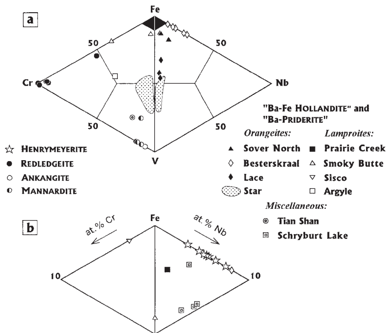
FIG. 3. Compositions (at.%) of cryptomelane-group titanate minerals in terms of different B-site cations (excluding Ti). (a) Quaternary plot in terms of Cr-Fe-Nb-V; (b) detailed view of the shaded area. This diagram incorporates only Ba-dominant compositions; priderite and structurally unassigned phases with K/Ba > 1.0 are not shown. Data corresponding to henrymeyerite are from this study; other data were taken from Gatehouse et al. (1986), Scott & Peatfield (1986), Mitchell & Meyer (1989), Xiong et al. (1989), Mitchell & Bergman (1991), Dmitriyeva et al. (1992), Platt (1994), Mitchell (1995), and Foley et al. (1997). Note that hollandite-type minerals from some localities, e.g., Murun and Pegmatite Peak (Mitchell & Vladykin 1993, Chakhmouradian & Mitchell 1999) lack detectable Cr, V and Nb; their compositions plot at the Fe apex of the diagram.
