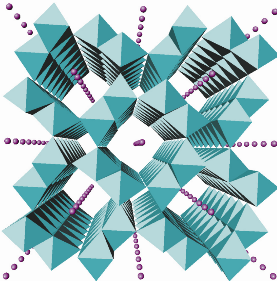
FIG. 2. Polyhedral representation of the structure of henrymeyerite, perspective view approximately along [001]. Note double-chain walls of (\text{Ti,Fe})\text{O}_6 octahedra (green) forming large and small square tunnels along [001]. Within the large tunnels, 2b positions partially occupied by Ba are denoted by purple circles.
