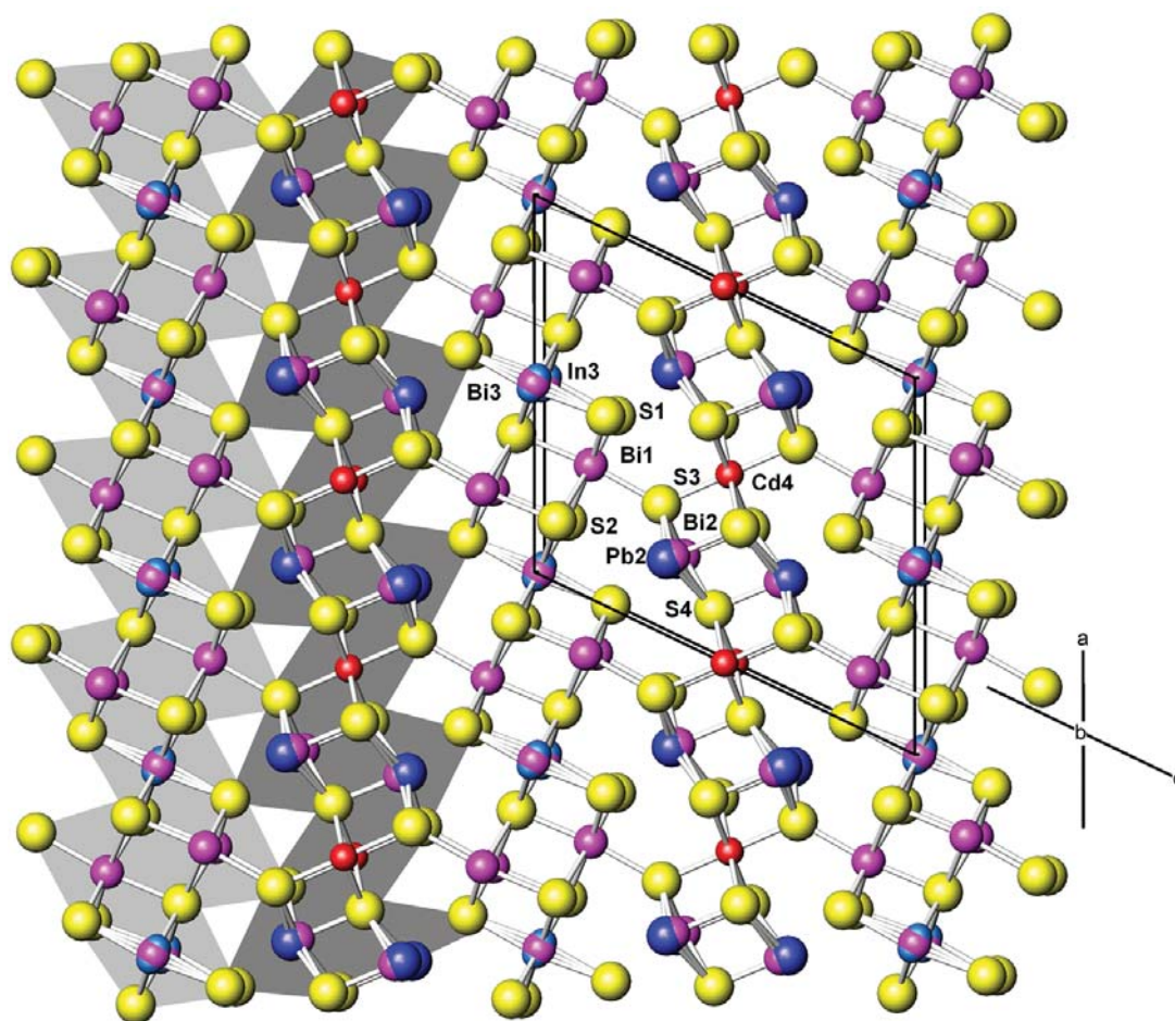
FIG. 1. Projection of the crystal structure of kudriavite. The characteristic structural slabs are marked by different background-shading on the left of the figure. Type-I slab has a darker background, and type-II slab has a lighter background. A trace of the unit cell and the labels of atoms in one asymmetric unit are also indicated.
