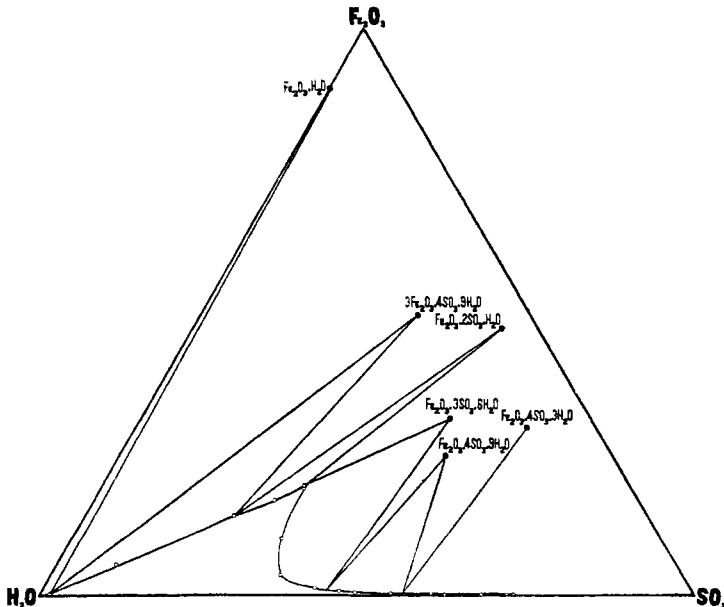
Fig. 6.—110° isotherm.
