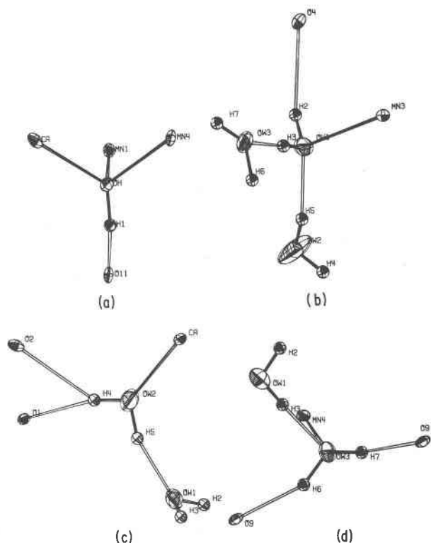
Fig. 4. Hydrogen bonding and the stereochemical configuration of the hydroxyl group and the water molecules in inesite.
