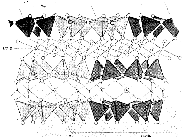
Fig. 2. An ac projection of the structure. At 1/2 c a portion of a Ca-octahedral sheet is outlined. Between the Si-O rings, at 1/4 c , the Li tetrahedra (solid circles), Ti octahedra (open circles), and K atoms (large open circles) are represented.
