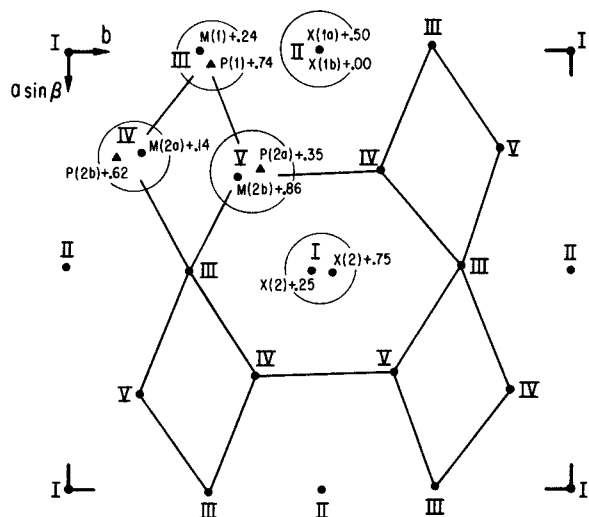
Fig. 3. The cations in the wyllieite structure (Moore and Molin-Case, 1974) with a portion of the \{6 \cdot 3 \cdot 6 \cdot 3\} and \{6 \cdot 6 \cdot 3 \cdot 3\} net drawn in. The structure is projected down [001] and preserves the axes and coordinates of the original study.
