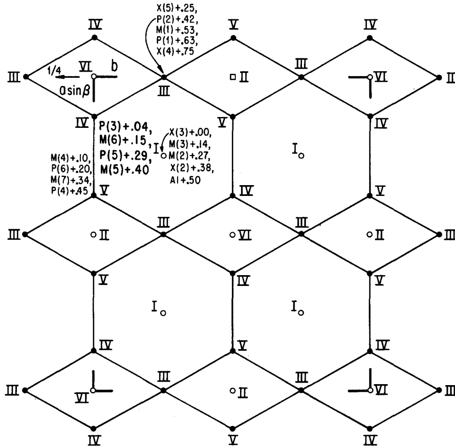
Fig. 2. Idealization of Figure 1 based on the (6 \cdot 3 \cdot 6 \cdot 3) and (6 \cdot 6 \cdot 3 \cdot 3) net constructed of rhombuses (two equilateral triangles with a common edge) and hexagons. The disordered cations P(1x), X(1), X(6) and X(7) have been left out. Note a c -glide plane occurs at b = 0 and a 2-fold rotor parallel to b at c = 1/4 . Open circles refer to inversion centers at z = 0, 1/2 .
