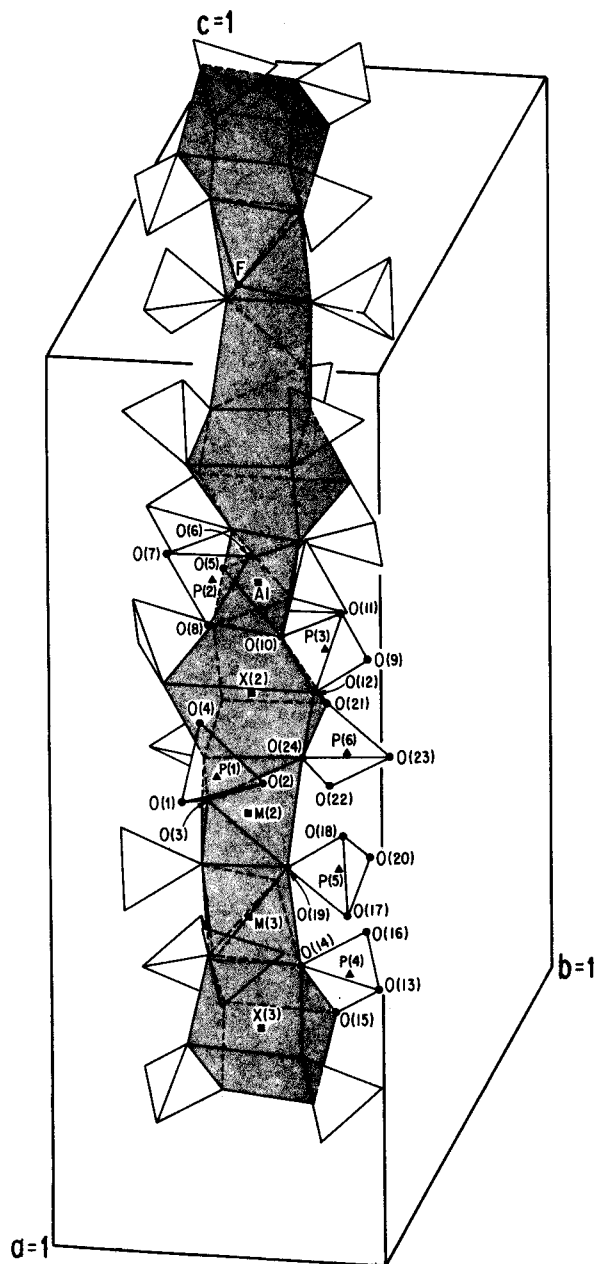
Fig. 4. Rod I in arrojadite (NM) drawn as a Penfield projection (Moore, 1981). The larger polyhedra are stippled and the enveloping transparent (PO_4) tetrahedra are drawn in. Note the sequence cube-octahedron-square pyramid-cube-octahedron-square pyramid-octahedron-cube. The Al site is an inversion center.
