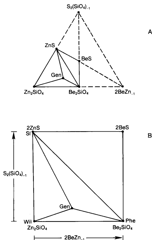
Fig. 1. Assumed mineral compatibilities in the reciprocal ternary system /Zn,Be//SiO_4,S/ . For abbreviations, see Table 1. (A) The composition triangle Zn_2SiO_4 - 2BeZn_{-1} - S_2(SiO_4)_{-1} . (B) The square defined by the exchange operators Be_2Zn_{-2} (or 2BeZn_{-1} ) and S_2(SiO_4)_{-1} as orthogonal vectors.
