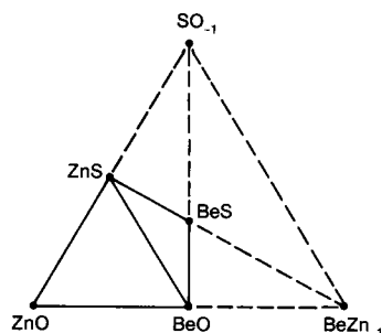
Fig. 2. Presumed low-pressure mineral compatibilities in the reciprocal system /Zn,Be//O,S/ , showing that Zn is more chalcophile than Be.
