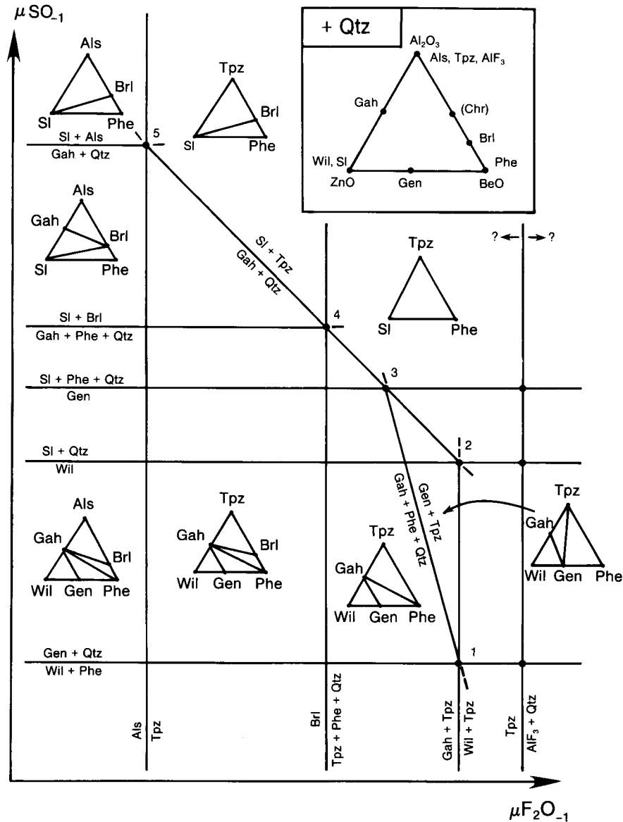
Fig. 11. Schematic isobaric, isothermal \mu_{SO_2} - \mu_{F_2O_3} diagram for the system ZnO - BeO - Al_2O_3 - SiO_2 - SO_2 - F_2O_3 , in the presence of quartz, at moderate temperatures and pressures. Genthelvite is assumed to be unstable with beryl. The five invariant points are numbered in order of increasing \mu_{SO_2} and decreasing \mu_{F_2O_3} , or \log a_{HF}^2/a_{H_2S} . Inset shows chemography of phases (see Tables 1 and 3 for abbreviations).
