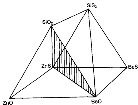
Fig. 4. System ZnO-BeO-SiO 2 -SO -1 (or /Zn,Be,Si/O,S/, written to show it is a reciprocal system) depicted as a triangular prism. The subsystem of interest, ZnO-BeO-SiO 2 -ZnS, is that to the left of the ruled plane.
