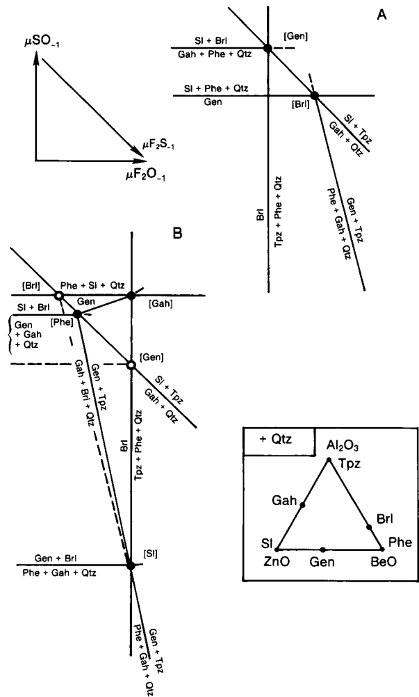
Fig. 12. Two alternative configurations for the multisystem derived from Reaction 4. Configuration A, to the upper right, is that of Fig. 11, in which the assemblage Gen + Brl is unstable. Configuration B, to the lower left, assumes that the assemblage Si + Gah + Phe + Qtz is unstable. See text for discussion; for abbreviations, see Tables 1 and 3.
