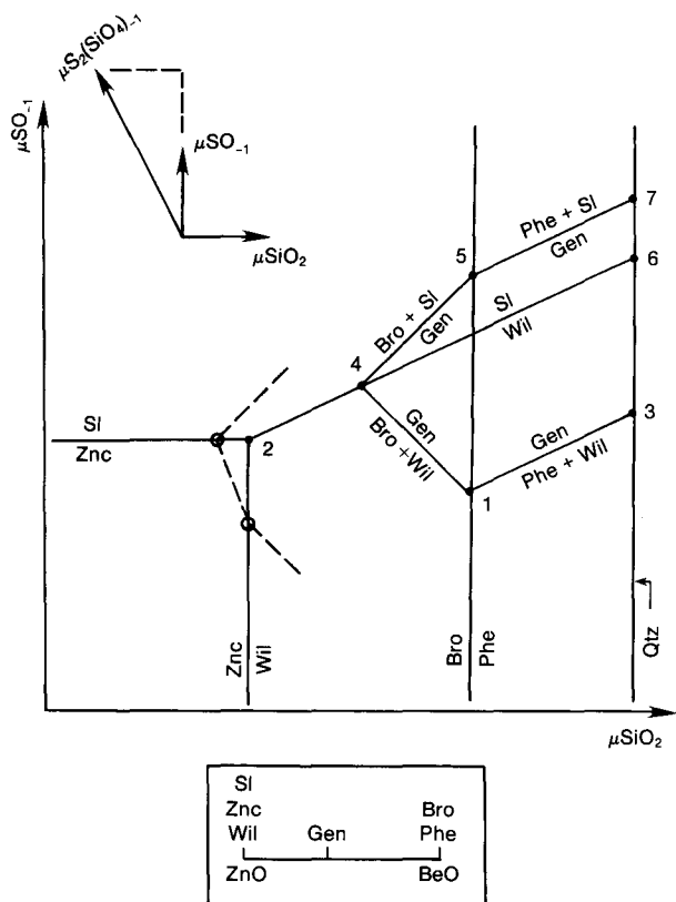
Fig. 7. Schematic isobaric, isothermal \mu_{SO_{-1}}-\mu_{SiO_2} diagram for the system ZnO-BeO-SiO_2-SO_{-1} , drawn at moderate temperatures and pressures, showing the stability of genthelvite in silica-saturated (vertical line to right) and undersaturated environments. For abbreviations, see Table 1.
