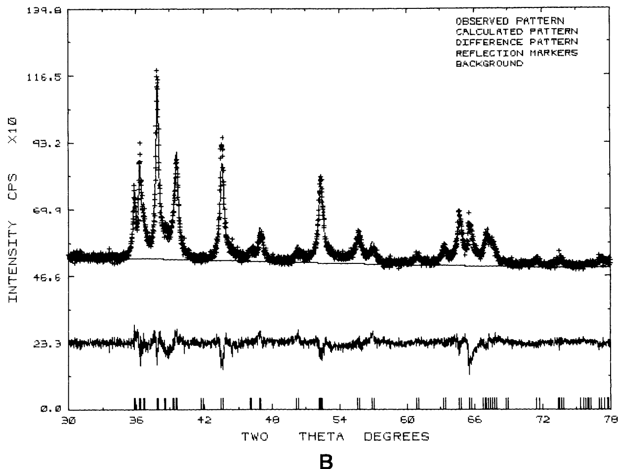
Fig. 8.—Continued. (B) Final observed (crosses) calculated, and difference powder XRD patterns for Mg-bir. See also Figures 8A and 8C.
