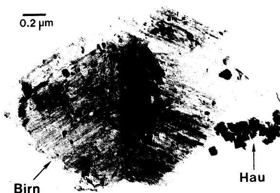
Fig. 2. TEM image of a typical twinned plate of Na-birn (Birn). Also shown are some crystals of hausmannite (Hau), which occurs as a minor impurity.
