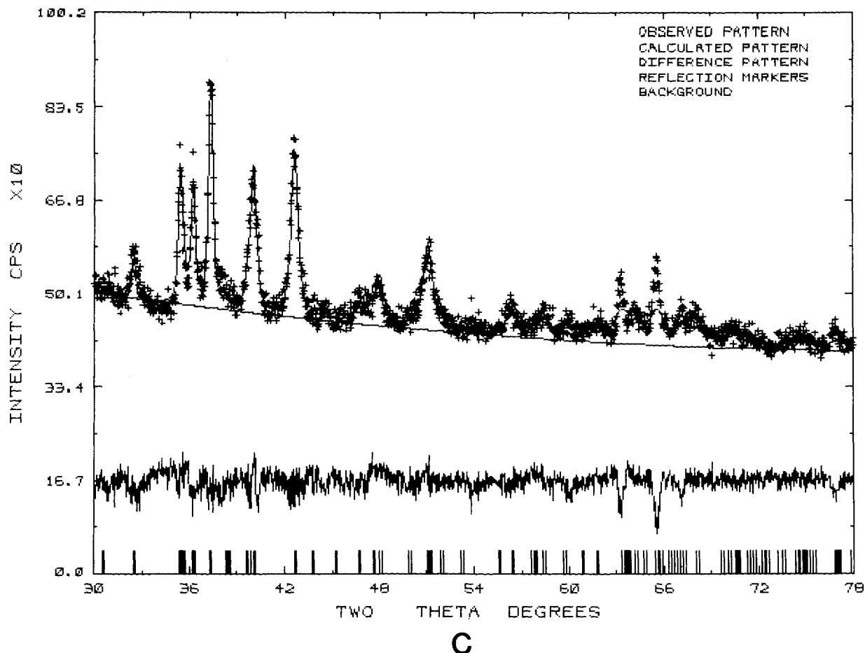
Fig. 8.— Continued. (C) Final observed (crosses), calculated, and difference powder xrd patterns for K-birn + hausmannite. See also Figures 8A and 8B.
