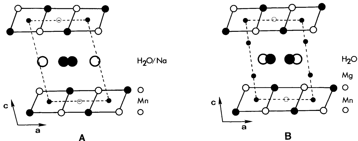
Fig. 9. Projections of the (A) Na-birn and (B) Mg-birn structures along b . The open circles indicate atoms at y = 1/2 , and the solid circles indicate atoms at y = 0 .
