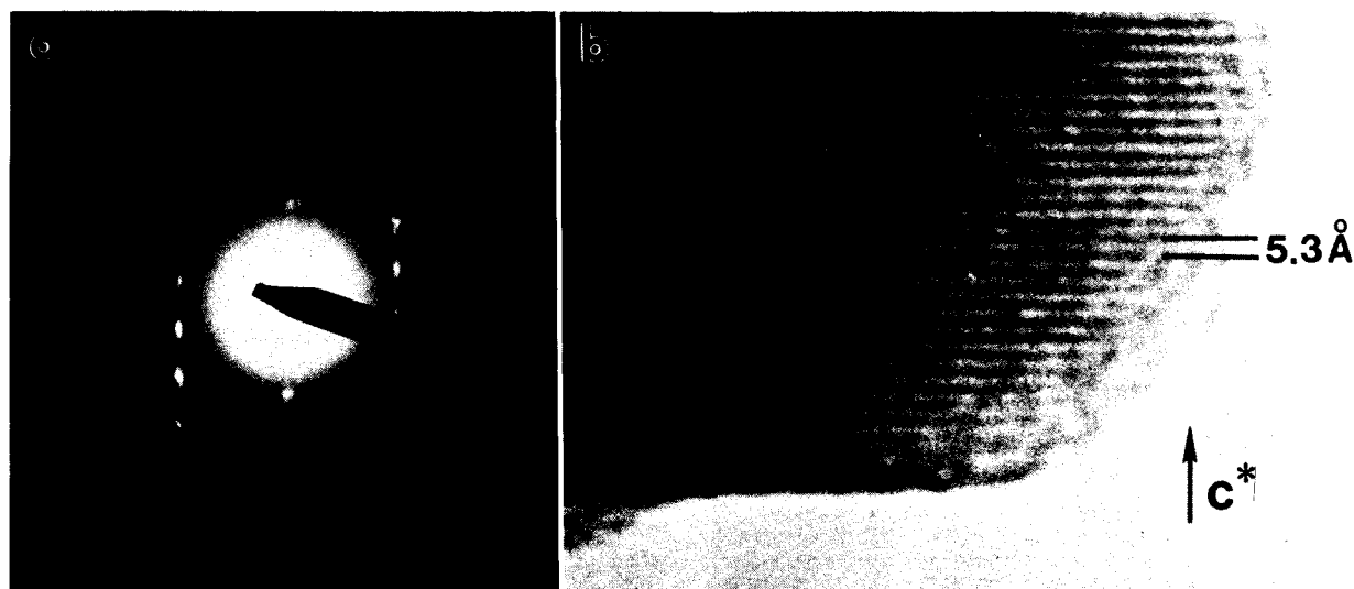
Fig. 5. (a) Selected-area electron-diffraction pattern and (b) high-resolution TEM image obtained from Na-birn with the electron beam parallel to the layers. This structure collapses in the vacuum of the electron microscope from an interlayer spacing of 7.1 Å to approximately 5 Å.
