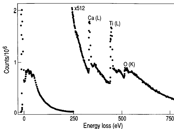
Fig. 2. EELS spectrum of kassite from Josephine Creek.
