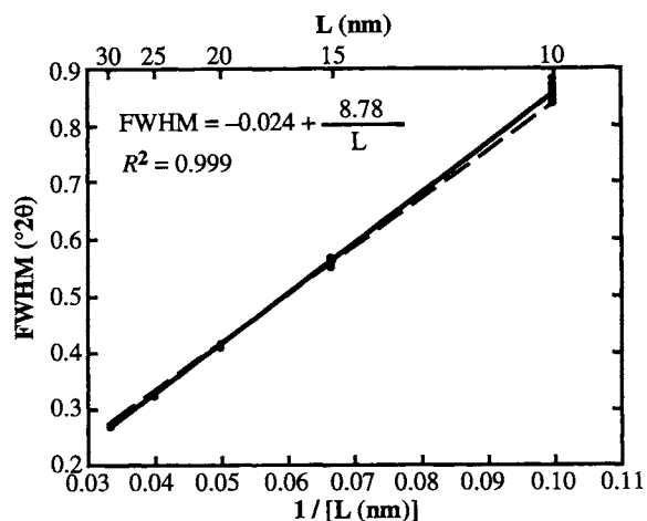
Fig. 2. Relationship between crystallite size ( L ) and calculated FWHM of the 35.9^\circ 2\theta peak. FWHM values taken from patterns calculated over the range in O_c (0.35–0.75) and P_{ud} (0.35–0.55) that is larger than the range we generally found for opal-CT. Crystallite size refers to the size along a or b . Equation in upper left represents a linear regression of FWHM to 1/L with units of degrees two-theta and nanometers. Equation does not take into account instrumental broadening effects; hence, observed FWHM values must be corrected for these effects before being used in this equation. For comparison with the Scherrer equation, we also fit the data using no intercept value and using units of radians and ångströms, which resulted in a K value of 0.907.
