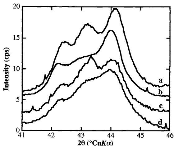
Fig. 3. Observed patterns for various opals, showing the weak intensity band in the 41–46° 2\theta region. (a) 28501; (b) 28781; (c) 114874; and (d) 46E5880. Step size was 0.04° 2\theta , and counting time was 600 s/step.
