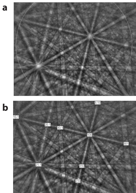
FIGURE 4. (a) EBSD pattern of the labeled \text{BaTiO}_3 crystal (upper one) in Figure 2b, (b) the pattern perfectly indexed with the \text{BaTiO}_3 Amm2 structure.
