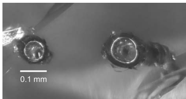
FIGURE 1. Photomicrograph of two hollow inclusions exposed at the surface of a polished crystal of benitoite. The left inclusion, which contains the barioperovskite , consists of a hollow core about 60 \mu\text{m} in diameter with a darker rim of mixed crystalline and amorphous material that ranges in thickness from 9 to 52 \mu\text{m} . The white ring at the immediate edge of the hollow core is an artifact from reflected light of the ring-illuminator used to illuminate the sample.
