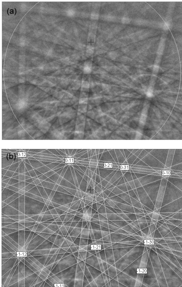
FIGURE 8. (a) EBSD pattern of sinoite in Zakłodzie. (b) The pattern indexed with the Cmc2_1 \text{Si}_2\text{N}_2\text{O} structure.
