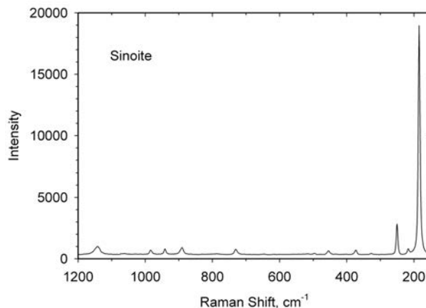
FIGURE 9. Raman spectrum of sinoite from the Zakłodzie meteorite.
