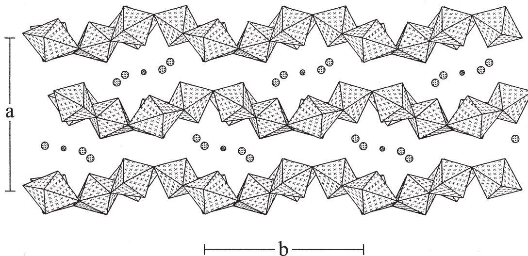
FIG. 3. The structure of curite projected onto (001). Large and small circles in the interlayer represent \text{Pb}^{2+} cations and \text{H}_2\text{O} groups, respectively.
