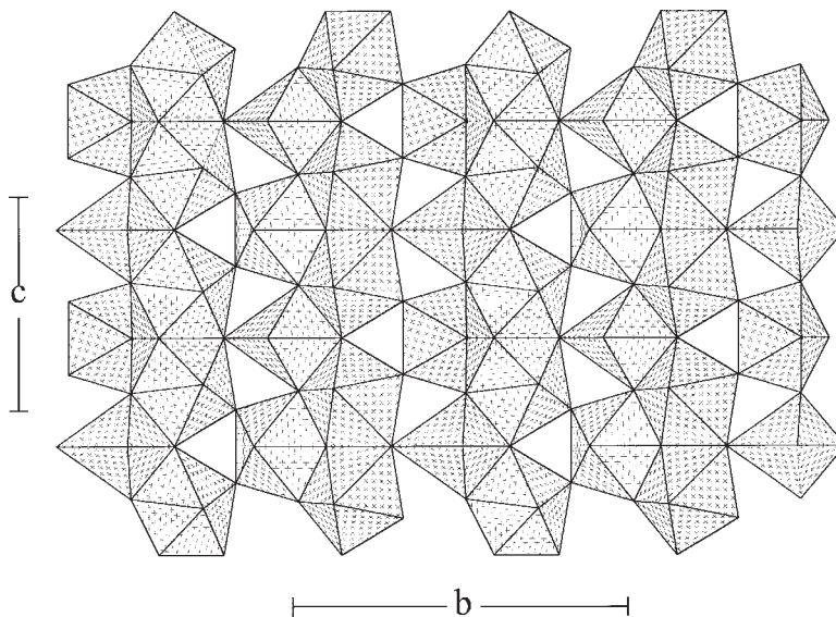
FIG. 2. The structural sheet in curite projected onto (100).
