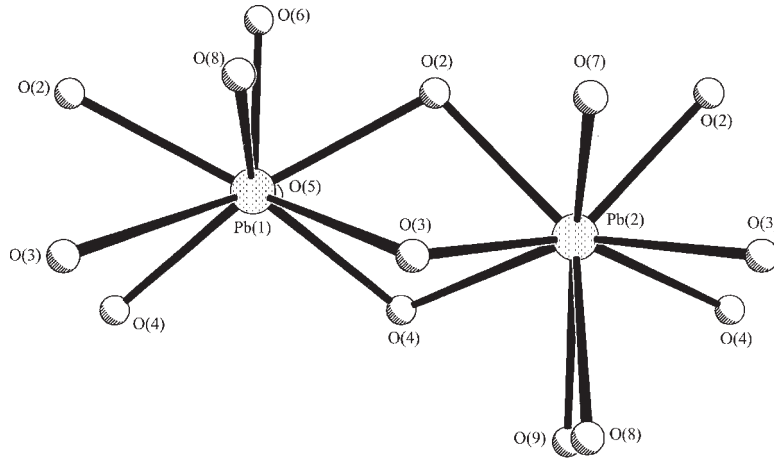
FIG. 1. Coordination environment about the \text{Pb}^{2+} cations in curite.
