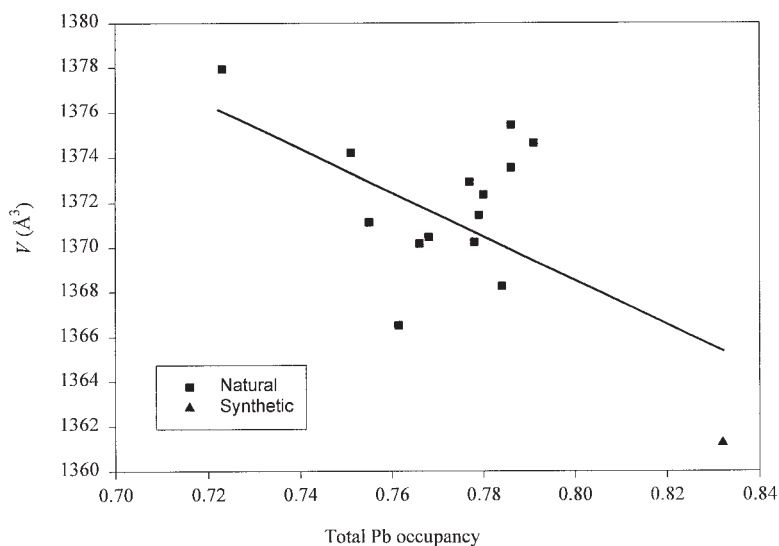
FIG. 4. Unit-cell volume versus total Pb occupancy obtained from crystal-structure refinements of fifteen crystals of curite. The line in the plot represents the result of linear regression of these data.
