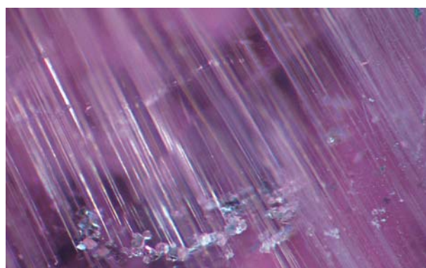
Figure 16. All of the pezzottaite samples examined contained numerous fine growth tubes oriented parallel to the c -axis. Some of the tubes shown here can be seen emanating from included crystals (identified as tourmaline). Photomicrograph by John I. Koivula; magnified 15 \times .
