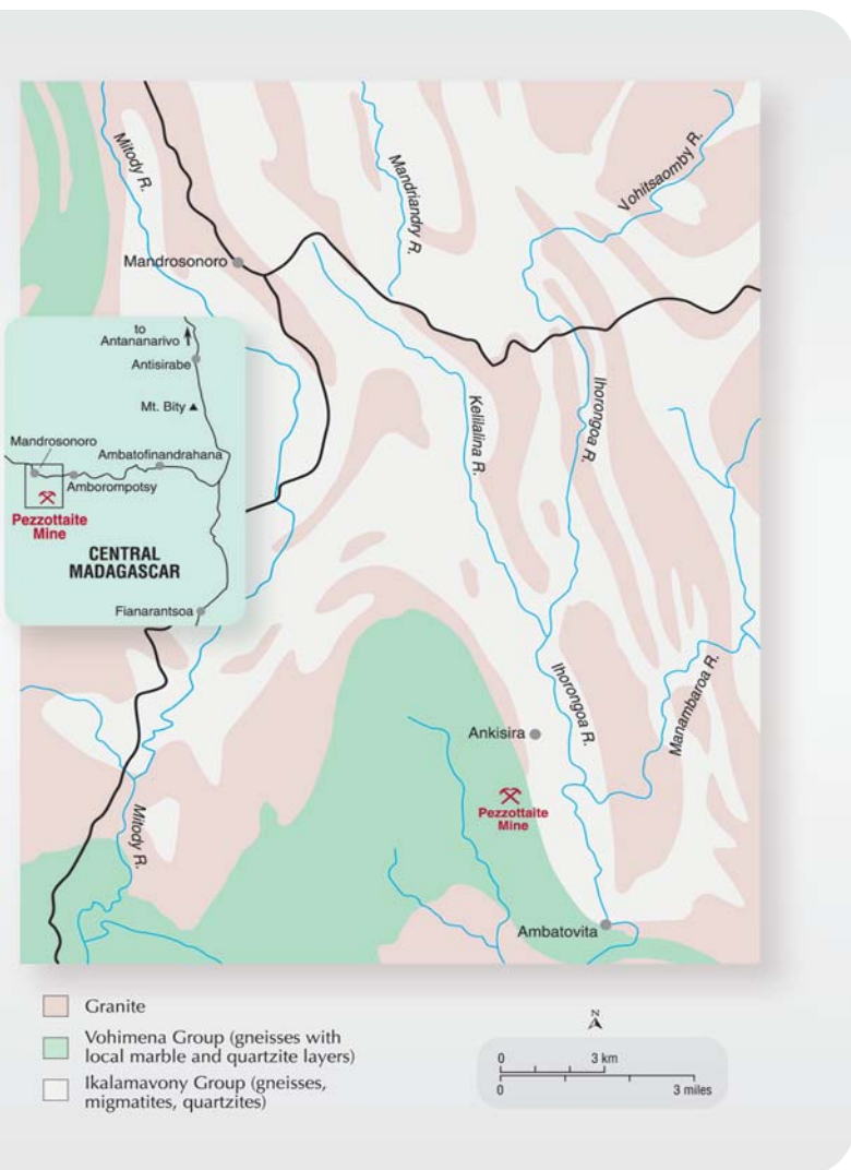
Figure 2. The pezzottaite deposit is located in central Madagascar, about 140 air-km southwest of Antsirabe and 130 km northwest of Fianarantsoa. From Antsirabe, a paved road leads south to Ambositra and west to Ambatofinandrahana, followed by a rough dirt track that passes through Amborompotsy and Mandrosonoro. The pegmatite is hosted by marbles, on the limb of a syncline that is composed mainly of quartzitic gneisses of the Vohimena Group. Geology from Chantraine (1966).
