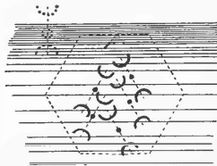
Fig. 7. Diagrammatic figure of the twin-formation in catapleite, type 2. The figure shows a part of the crystal where two individuals alternate with each other; here the lines show the boundaries between the individuals. In the upper part of the figure the individuals become so narrow, that they cannot be distinguished from each other under the microscope; consequently the two axial planes become one, which is designated by the dotted axial figure.
