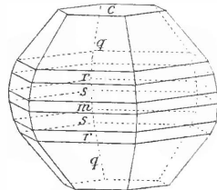
Fig. 3. Cordylite; Narsarsuk.
