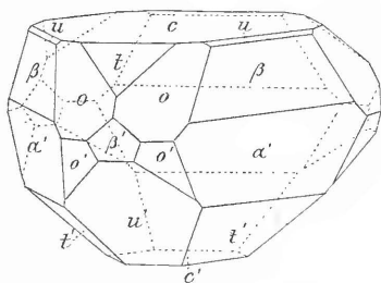
Fig. 2. Synchysite; Narsarsuk.
