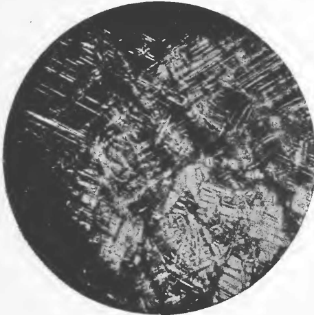
Fig. 9. Microscopical section of catapleite type 3. The twin-formation is as shown diagrammatically in fig. 8. The boundary line above represents a surface of m\{10\bar{1}0\} . The enlargement 1:45; after a photograph by K. J. V. Steenstrup.
