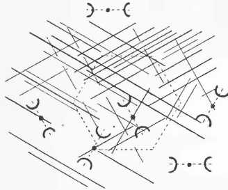
Fig. 8. Diagrammatic figure of the twin-formation in catapleite, type 3. The explanation chiefly as in fig. 6.
