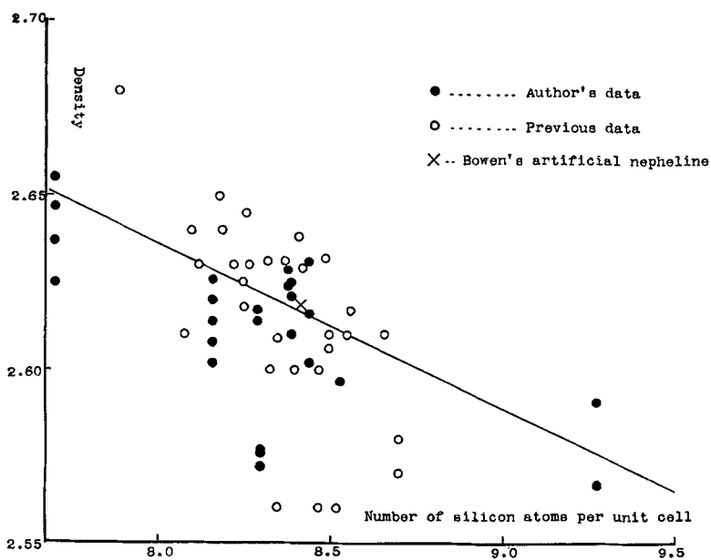
Fig. 2. Graph plotting the number of silicon atoms per unit cell against the density of nepheline. Series of points falling on the same ordinate give the density of individual crystals taken from each analysed specimen.
