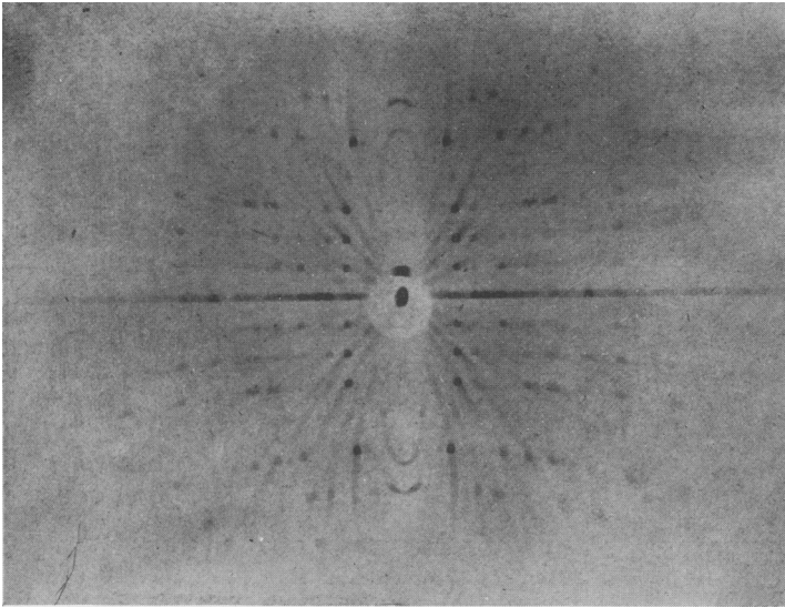
FIG. 9. Rotation photograph of nepheline specimen no. VI (crystal 2) about the c -axis.
