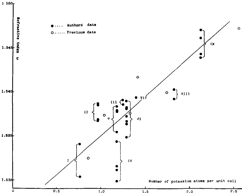
FIG. 4. Graph plotting the number of potassium atoms per unit cell against the refractive index ( \omega ) of each crystal of nepheline measured.
