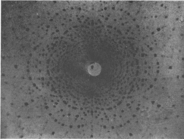
FIG. 7. Laue photograph of nepheline specimen no. V1 (crystal 2) perpendicular to the c -axis and with an a -axis horizontal.
