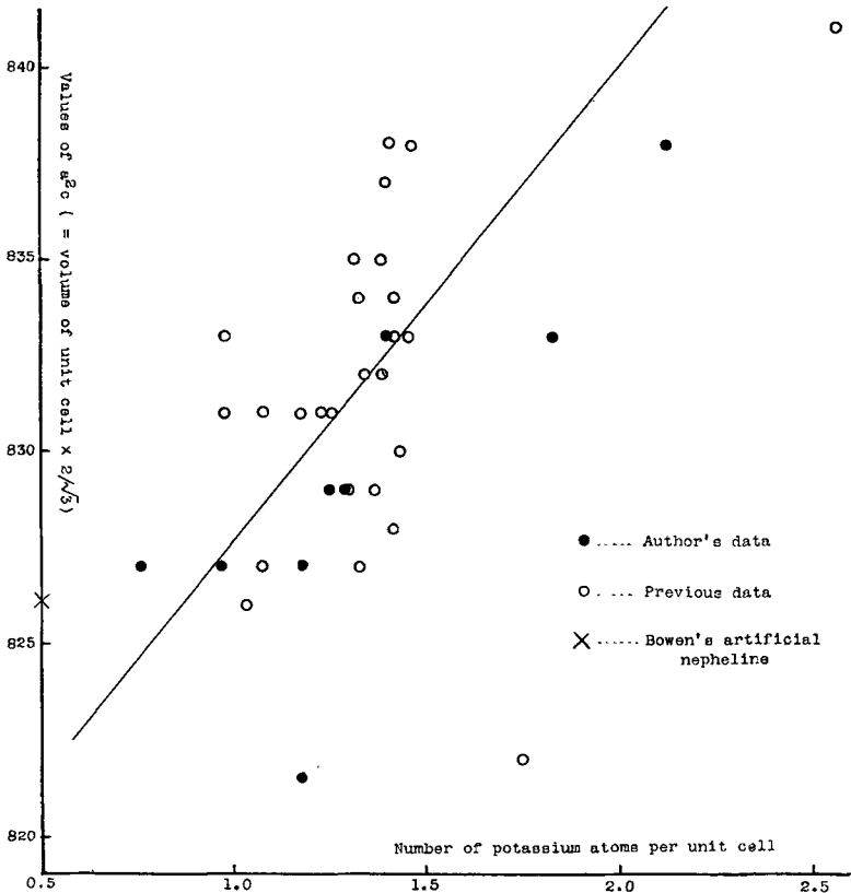
FIG. 3. Graph plotting the number of potassium atoms per unit cell against the cell-volume \times 2/\sqrt{3} . (Only the author's data, represented as black spots, were obtained directly by X-ray methods.)
