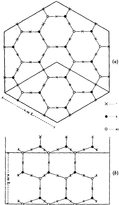
FIG. 5. Two views of the scaffolding of the nepheline structure: (a) perpendicular to the c -axis; (b) perpendicular to an a -axis.
