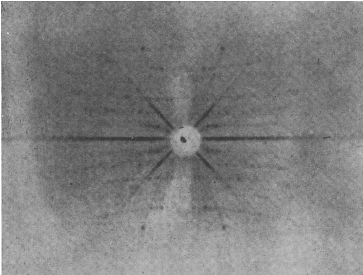
FIG. 10. Rotation photograph of kaliophilite specimen no. X about the c -axis.
