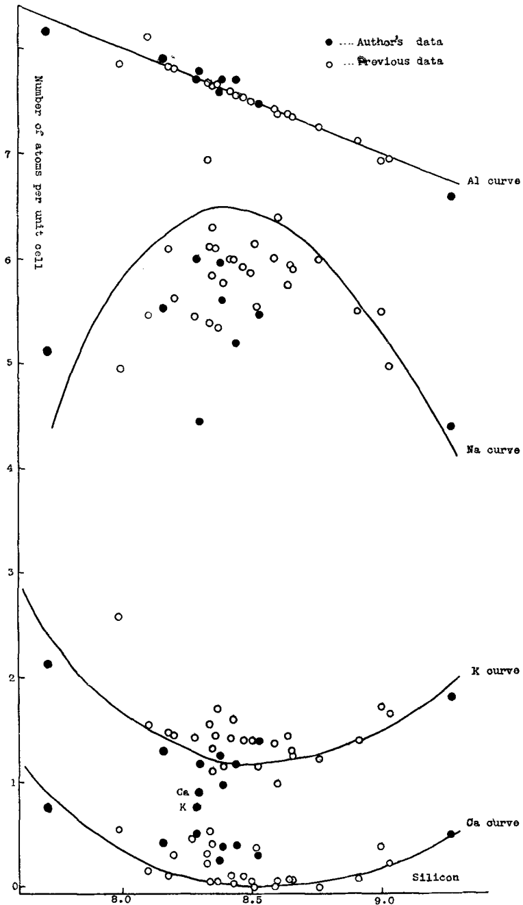
FIG. 1. Graphs plotting number of silicon atoms per unit cell of nepheline against number of aluminium, sodium, potassium, and calcium atoms per unit cell.
