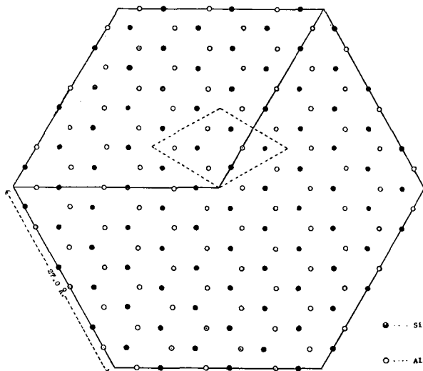
FIG. 6. Plan of a possible kaliophilite scaffolding built up from nepheline cells. The dotted outline is a nepheline unit cell.
