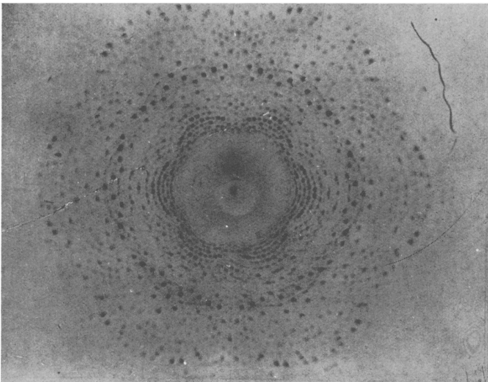
FIG. 8. Laue photograph of kaliophilite specimen no. X in same orientation as the nepheline specimen (fig. 7).
