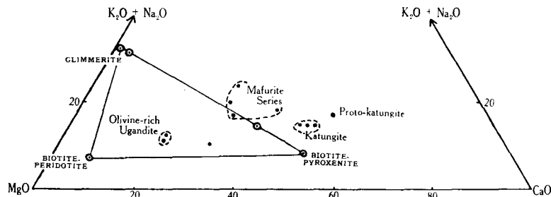
FIG. 3. Triangular diagram (in terms of MgO, CaO, and alkalis) showing the relationships of the volcanic types of Bunyaruguru to the associated cognate plutonic types.
