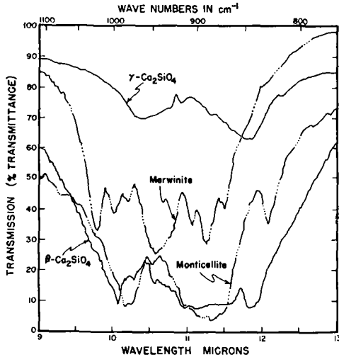
FIG. 2. Infra-red absorption spectra. Monticellite and \beta\text{Ca}_2\text{SiO}_4 obtained using 0.4% concentration in KBr pellet, merwinite 0.2% in KBr; \gamma\text{-Ca}_2\text{SiO}_4 obtained from 'Nujol' mull on NaCl plates.
