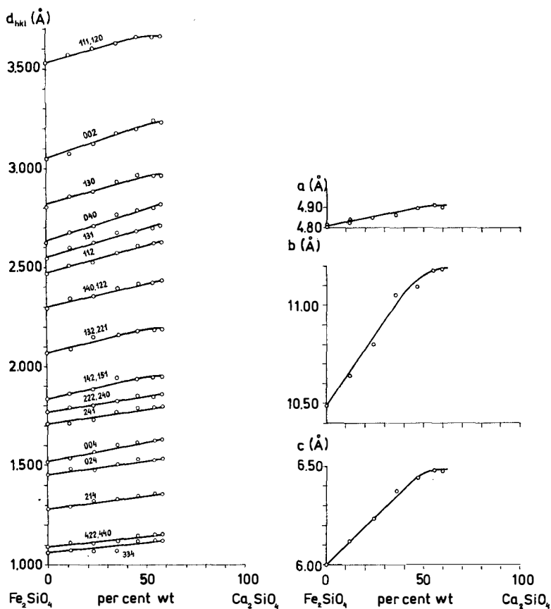
FIGS. 2 and 3: FIG. 2 (left). Correlation of the spacings of various planes hkl with the composition of calcium-iron olivines. FIG. 3 (right). Correlation of the cell-dimensions with the composition of calcium-iron olivines.
