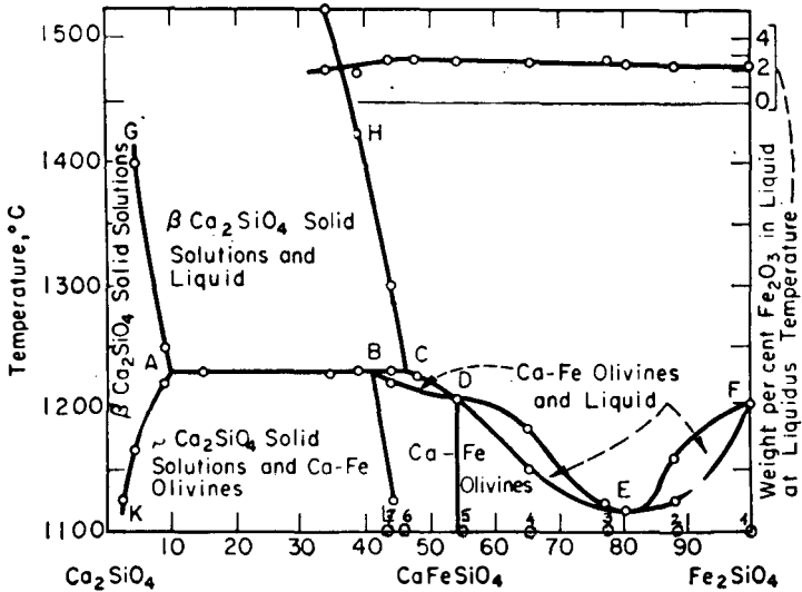
FIG. 1. \text{Ca}_2\text{SiO}_4 - \text{Fe}_2\text{SiO}_4 phase diagram after Bowen, Schairer, and Posnjak. The numbered points 1 to 7 indicate the assumed compositions of the olivines examined.
