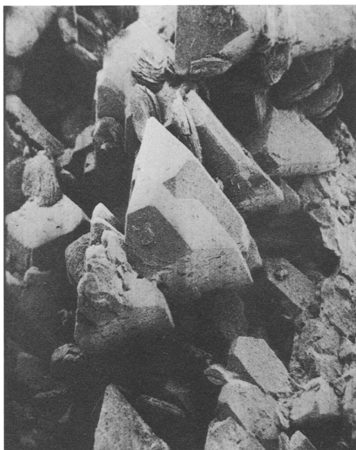
FIG. 1. Scanning electron micrograph ( \times 70 ) showing a pseudotrigonal contact triplet.
