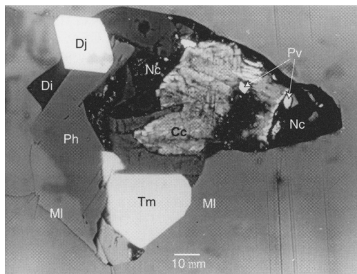
FIG. 1. Two micro-inclusions from melilite showing djerfisherites (Dj) and a range of other daughter minerals. Note the heterogeneous distribution of phases in individual sections through the inclusions. Abbreviations: MI – melilite; Di – diopside; Ph – phlogopite; Tm – titanomagnetite; Pv – perovskite; Ap – apatite; Cc – calcite; Nc – Na-K-rich carbonate.
