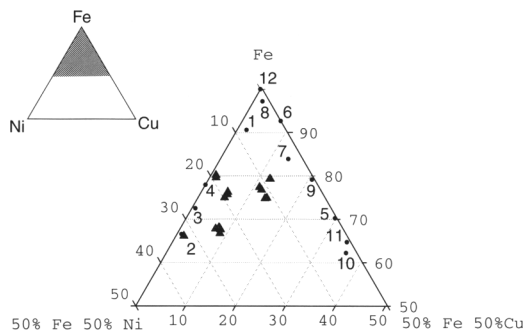
FIG. 2. Fe-Cu-Ni composition variations (at. %) in djerfisherites from Kugda (solid triangles) and other igneous localities (small solid symbols with numbers as in Table 2). Note that the most Ni-rich djerfisherites from Kugda have similar compositions to samples from kimberlites.
