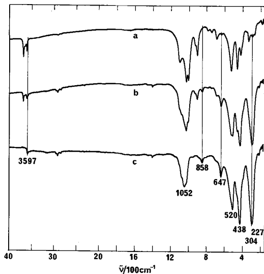
FIG. 2. Infra-red spectra of macaulayite in (a) untreated < 2 \mu\text{m} clay with kaolinite impurity, (b) electromagnetically concentrated fraction of < 2 \mu\text{m} clay, (c) computer-generated difference spectrum between magnetic concentrate and < 2 \mu\text{m} clay.
