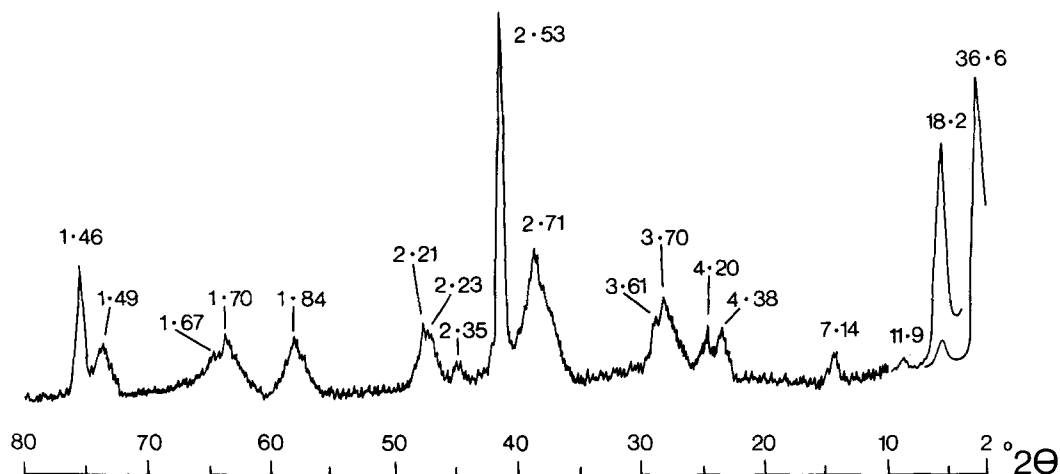
FIG. 1. Diffractometer pattern of macaulayite obtained with Co-K \alpha radiation, 40 kV 35 mA, using an oriented aggregate from 2 to 10° 2 \theta and a randomly ordered powder from 10 to 80° 2 \theta . Divergence, receiving, and antiscatter slits as follows: 2–5° 2 \theta , \frac{1}{4}^\circ , 0.1 mm, \frac{1}{4}^\circ ; 5–10° 2 \theta , \frac{1}{2}^\circ , 0.1 mm, \frac{1}{2}^\circ ; 10–80° 2 \theta , 1°, 0.2 mm, 1°.
