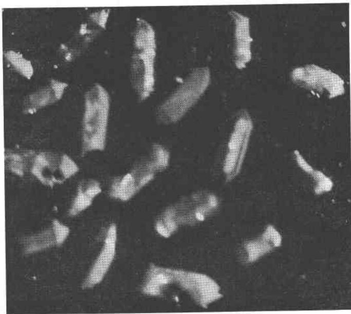
FIG. 3 Doubly terminated quartz crystals from the sandstone member of the Jonesboro formation. Magnified 5 times.
