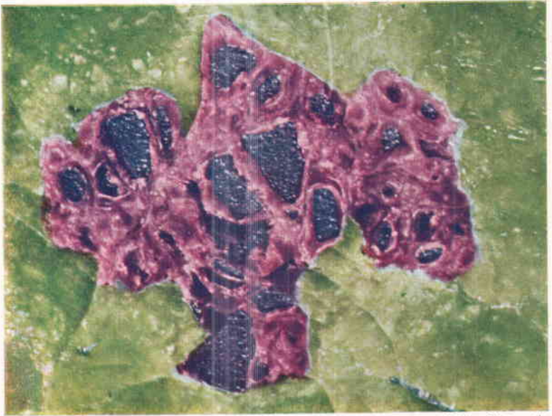
Serpentine with stichtite surrounding chromite from near Dundas, Tasmania. \times = 16
