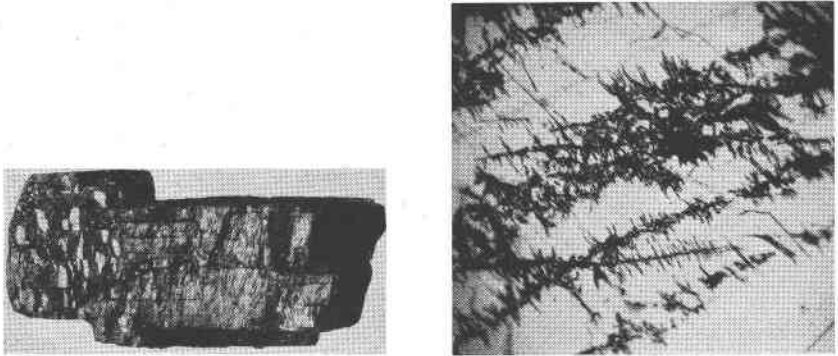
FIG. 2. Specimen of pinite after cordierite, showing development of micaceous blades normal to the {001} parting of the cordierite. Length of specimen is seven inches. Climax pegmatite, Colo.
