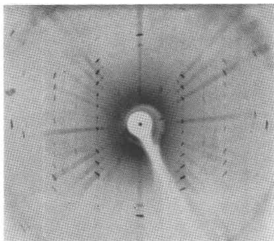
FIG. 4. Buerger precession photograph of (h0l) net plane of smythite. MoK radiation, unfiltered.
