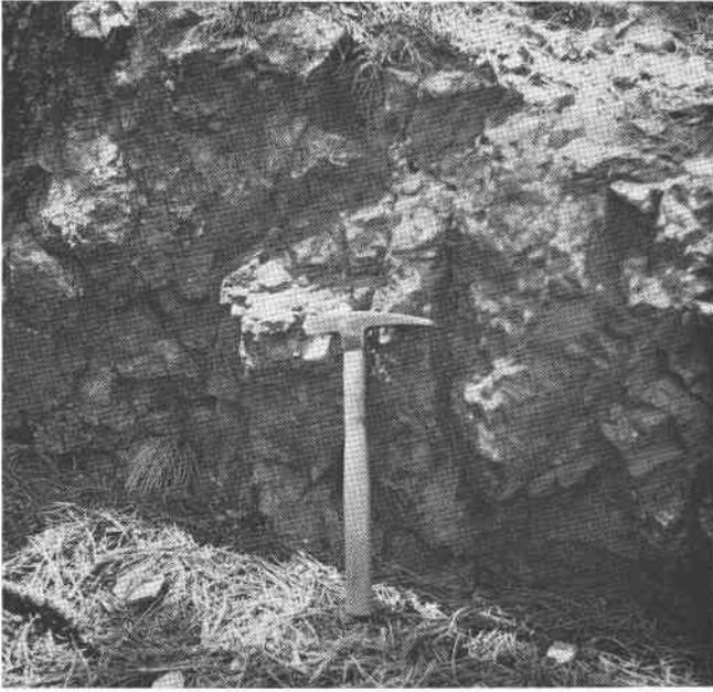
FIG. 4. Close-up view of riebeckite crystals (above and right of hammer) in microcline-quartz rock of Mt. Rosa pegmatite.
