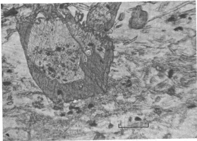
FIG. 2. Basal section of amphibole showing pale green actinolite sharply demarcated by green hornblende rim. Scale 0.1 mm.
