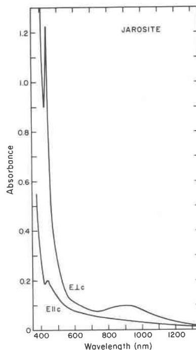
FIG. 6. Optical absorption spectrum of a jarosite crystal 22 \mu\text{m} thick from Pershing County, Nevada.
