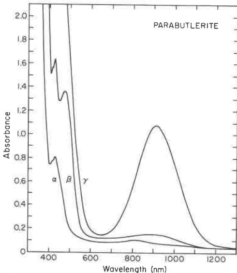
FIG. 2. Optical absorption spectrum of a parabutlerite crystal illustrating the enhancement of the first absorption band of \text{Fe}^{3+} at 912 nm in \gamma -polarization and the 478 nm \beta -feature; crystal 300 \mu\text{m} thick from Yazd, Iran.
