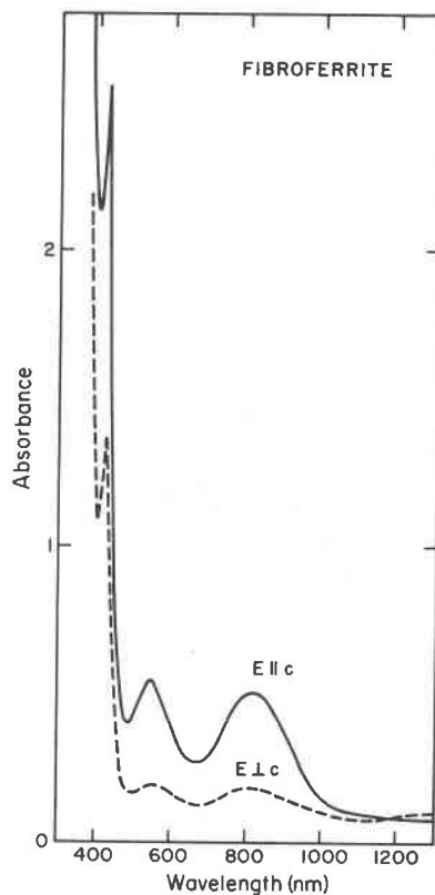
FIG. 5. Optical absorption spectrum of a bundle of fibroferrite fibers 250 \mu m thick soaked in a liquid with n_D = 1.54 (specimen from Cyprus).
