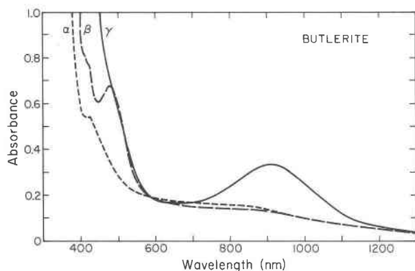
FIG. 3. Optical absorption spectrum of a butlerite crystal 106 \mu\text{m} thick from Jerome, Arizona.
