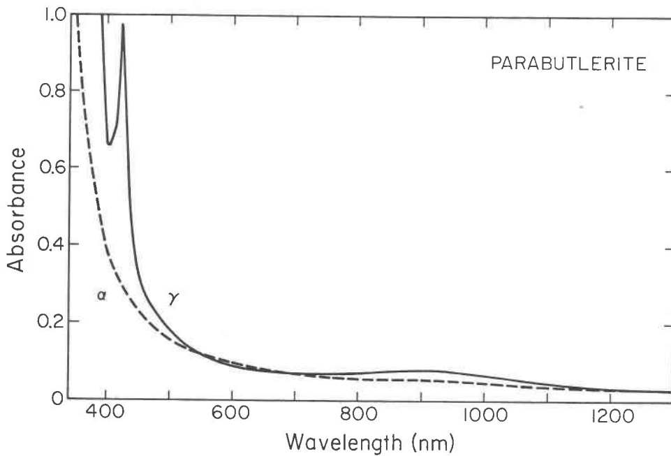
FIG. 1. Optical absorption spectrum of a parabutlerite crystal 20 \mu\text{m} thick from Yazd, Iran, showing the intense absorptions in \gamma -polarization.
