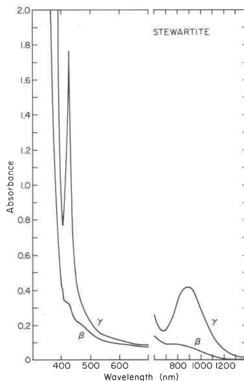
FIG. 4. Optical absorption spectrum of a stewartite crystal showing enhanced \text{Fe}^{3+} absorption bands and \text{Mn}^{2+} bands without enhancement. Crystal from the Fletcher Pegmatite, N. Groton, N. H.: for \lambda = 300\text{--}700 nm, 22 \mu\text{m} thick; for \lambda = 700\text{--}1400 nm, 150 \mu\text{m} thick.
