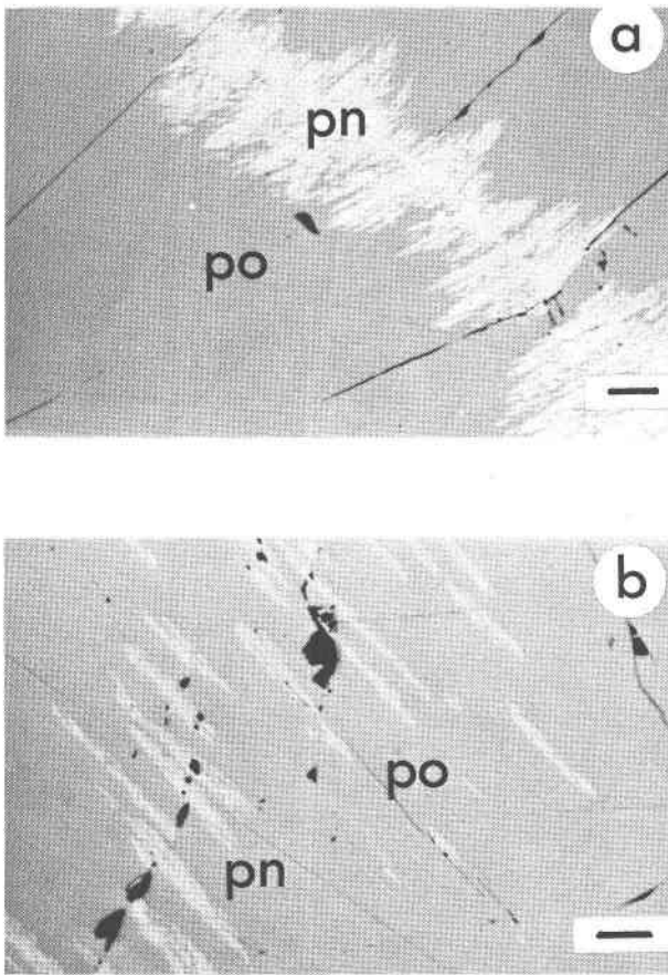
FIG. 1. Photomicrographs illustrating some typical pentlandite (pn)–pyrrhotite (po) textural relationships. The bar in each photomicrograph represents 0.04 mm. Oil immersion, reflected light.
