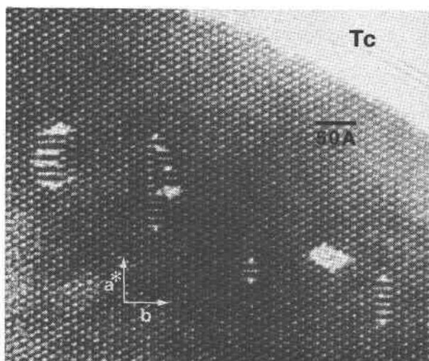
Fig. 17. Copper Mountain uralite. Short, double-terminated zippers of wide-chain silicate growing in amphibole near a grain boundary filled with talc. Two of the zippers are simple, consisting purely of sextuple-chain material, while the other two are complex, consisting of silicate with double, triple, and wider chains.
