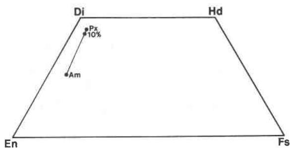
Fig. 31. Error introduced by analyzing pyroxene containing 10% amphibole lamellae, assuming theoretical cation partitioning behavior (see text).
