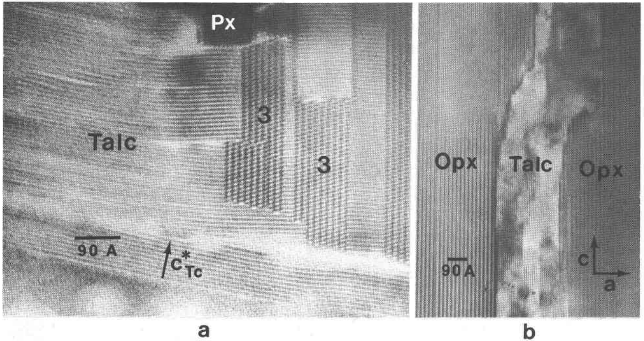
Fig. 5. Palisades augite. (a) Complex intergrowth of pyroxene, talc, and triple-chain silicate ("3"). (b) Direct replacement of orthopyroxene by talc along a fracture.
