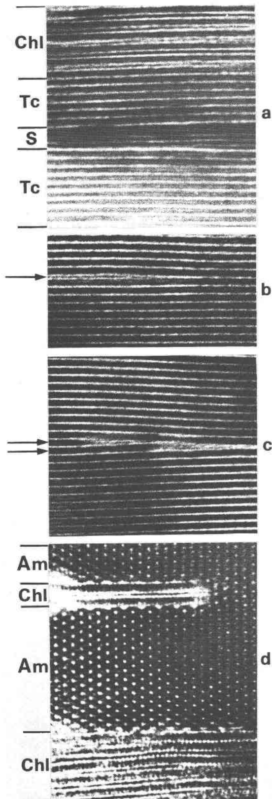
Fig. 19. Copper Mountain uraltite. Sheet silicates intergrown on (001); c^* is vertical, and fringe spacing in the talc regions is 9.3 Å. (a) Intergrowth of chlorite, talc, and planar serpentine structures. (b) Intercalation and termination of a 5 Å brucite layer (arrowed) in talc. The intercalation is structurally equivalent to the insertion of one layer of chlorite structure. (c) The termination by dislocation of two talc layers (arrowed). (d) Chlorite intergrown with amphibole. A short chlorite sequence consisting of talc-brucite-talc layers terminates in the upper portion of the figure.
