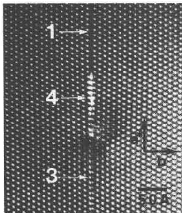
Fig. 18. Copper Mountain uraltite. A low-angle grain boundary separating two amphibole domains parallel to (010). The structural misfit is accommodated by distortion and changing of the chain width of the boundary from single ("1") to quadruple ("4") to triple ("3").
