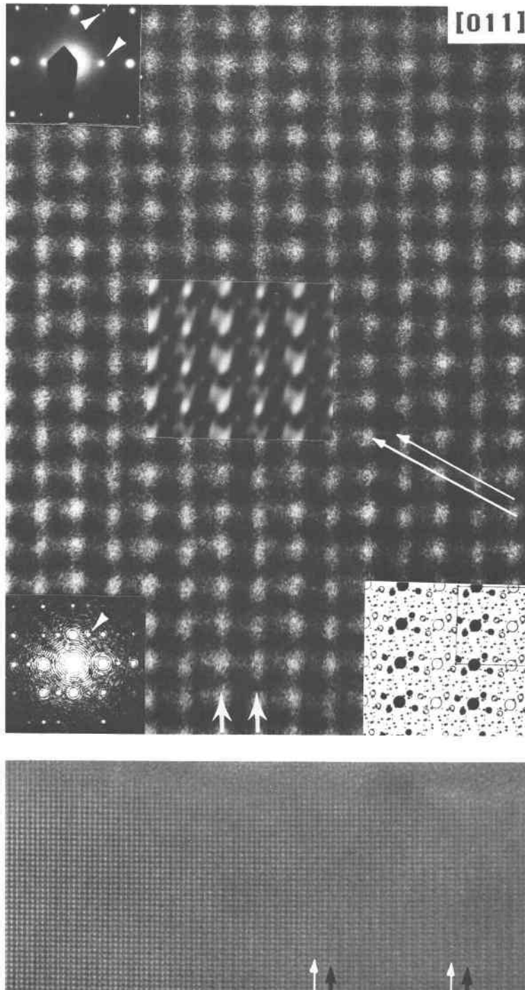
Fig. 8. A [011] HRTEM image (top) and low-magnification image (bottom) of the Mc_{39.5} sample. Inserts of the SAED pattern and optical diffractogram are given in the upper- and lower-left corners, respectively, in the image at the top. The calculated image in the central insert is based on the ordered model ( H = 51.4 \text{ \AA} , \Delta f = -800 \text{ \AA} ; cf. Fig. 3d). Ordering of [\text{Na}_4\text{Cl}]^{3+} and [\text{NaCa}_3\text{CO}_3]^{5+} clusters is indicated in the projected structure (lower-right corner; the a axis is horizontal and [011] is vertical) and is more evident in the image shown at the bottom in which white and black arrows point out rows that have light and dark contrast, respectively.
