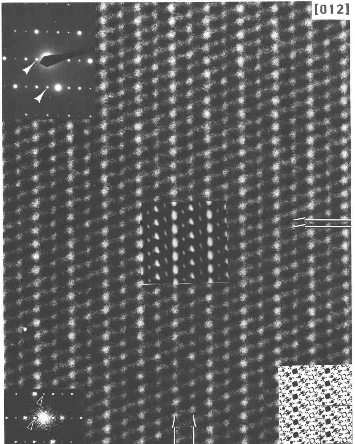
Fig. 7. A [012] image of the Me_{39.5} sample. The SAED pattern and the optical diffractogram are shown as inserts at the upper- and lower-left, respectively. The simulated image in the central insert is based on the ordered model ( H = 75.9 \text{ \AA} , \Delta f = -1200 \text{ \AA} ; cf. Fig. 3c). The projected structure (lower right; the a axis is horizontal and the [02\bar{1}] axis is vertical) shows ordering of [\text{NaCa}_3 \cdot \text{CO}_3]^{2+} and [\text{Na}_4 \cdot \text{Cl}]^{3+} clusters that is evident in the image.
