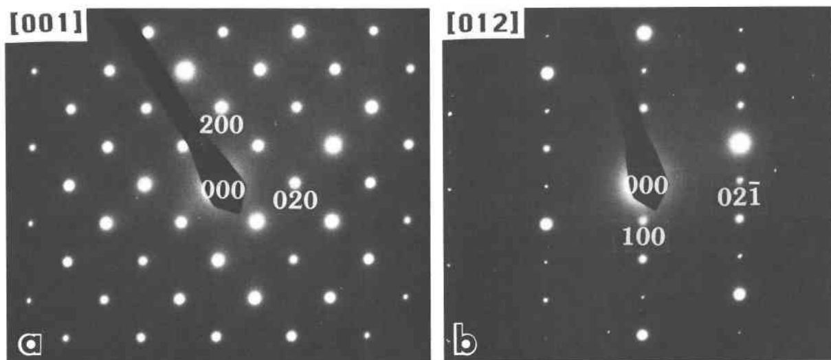
Fig. 5. (a) A [001]-zone SAED pattern showing type a reflections. (b) A [012]-zone SAED pattern for the \text{Me}_{39.5} sample showing strong type b (e.g., 02\bar{1} , 142 , 22\bar{1} , 142 ) and type d (e.g., 100 , 300 , 500 ) reflections.
