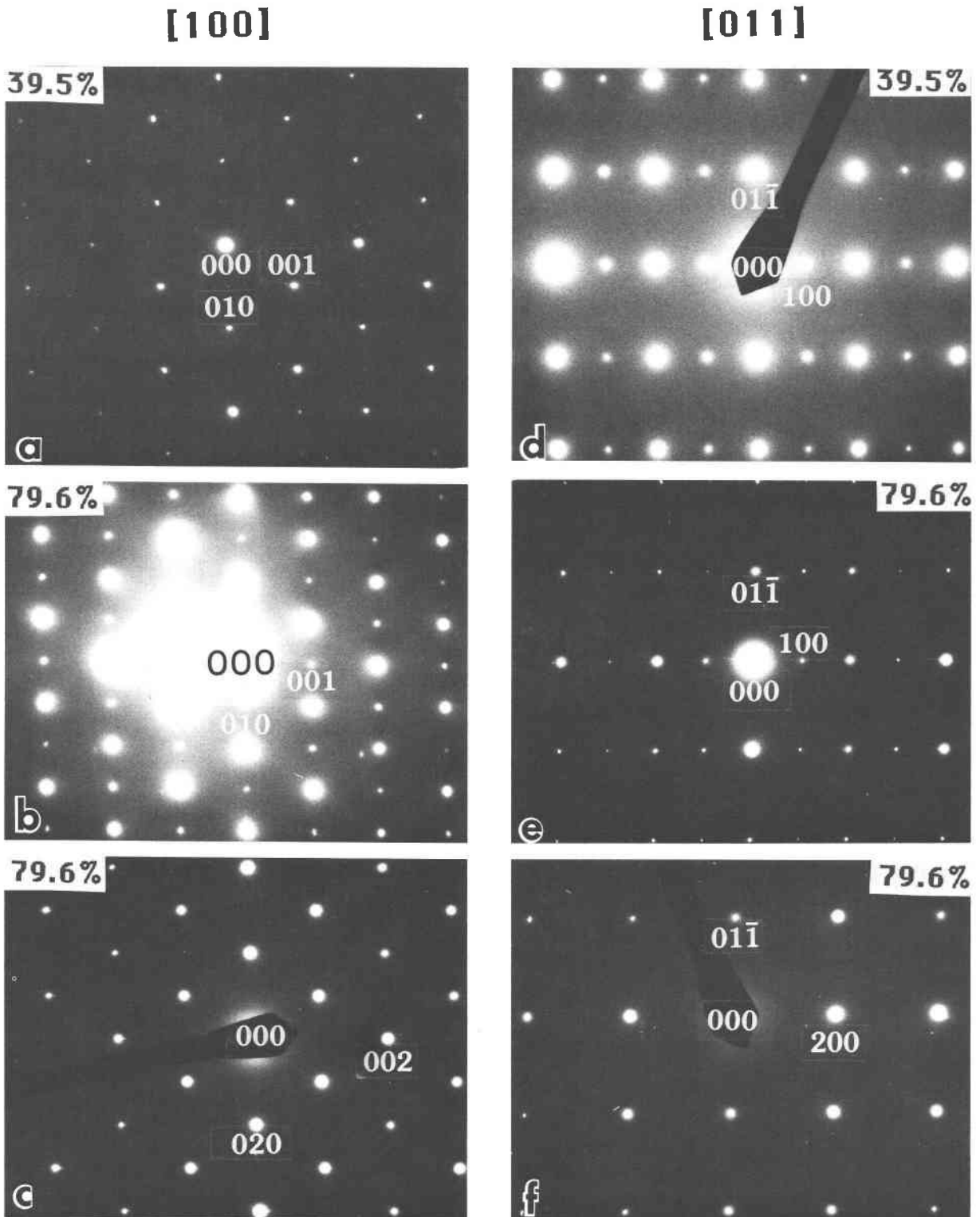
Fig. 6. Comparison of [100] (Figs. 6a, 6b, 6c) and [011] (Figs. 6d, 6e, 6f) SAED patterns for \text{Me}_{39.5} (Figs. 6a, 6d) and \text{Me}_{79.6} (Figs. 6b, 6c, 6e, 6f). Reflections of the following types are shown: type b (Figs. 6a, 6b contain 021 , 012 , 014 , 032 , etc.; Figs. 6d, 6e contain 11\bar{1} , 122 , etc), type c (Figs. 6a, 6d contain 001 , 003 , etc.), and type d (Figs. 6d, 6e contain 100 , 300 , etc.). These reflections are absent in some crystal fragments of the \text{Me}_{79.6} sample (Figs. 6c, 6f).
