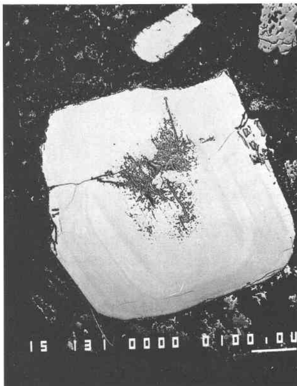
Fig. 6. BSE image of a partially altered plagioclase phenocryst from sample 212J. Scale bar is 100 \mu m. The core of the plagioclase has been extensively altered, and replacement has taken place by the development of a vermicular texture, with abundant narrow tubes. Locally, where cracks extend to the rim, alteration is more extensive, indicating that the cracks acted as pathways for infiltrating fluids.
