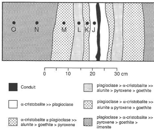
Fig. 1. Schematic map showing the location of samples J–O in dacite rich ash-flow tuff in the region of the fossil fumarole conduit. The relative abundance of the crystalline phases, as determined by optical petrography, in the nearly symmetric alteration zones adjacent to the conduit are noted. Encrusting minerals, characteristic of the upper surface region of the fissure fumaroles at Katmai, have been removed by erosion. (After Papike et al., 1991b.)
