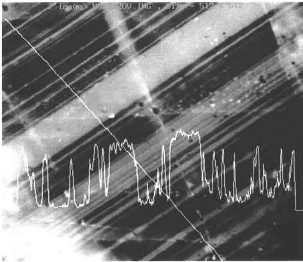
Fig. 1. Cathodoluminescence image of oscillatory zoning in a zircon crystal from Silinjärvi, Finland; dark regions show green luminescence, and light regions show pale yellow luminescence. The field of view is 1000\ \mu\text{m} , and the zones vary in width from 5 to 150\ \mu\text{m} . The overlay (white lines) shows (1) the traverse over which the information was collected (from top left to bottom right); (2) the gray-level variation with respect to position over the length of the traverse. The irregular bright region in the lower left of the picture is light scattered from a fracture outside the field of view.
