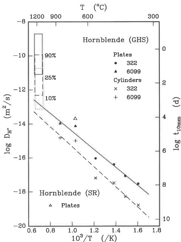
Fig. 6. A plot of H diffusivity vs. temperature for pargasitic hornblende using the data of Graham et al. (1984) (GHS) and a value inferred from the observations of Skogby and Rossman (1989) (SR). The boxes in the upper left of the figure show the diffusivities necessary to produce the percentage indicated of H loss for 10-mm hornblendes over the temperature range from 1100 to 1250 °C on a time scale of 3 h to 30 d.
