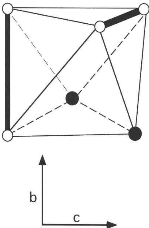
Fig. 8. The ^{[6]}\text{Al} coordination polyhedron. Bold lines are O-O edges shared with adjacent octahedra; solid circles represent F atoms, and open circles are O atoms. Al in the center is not shown.
