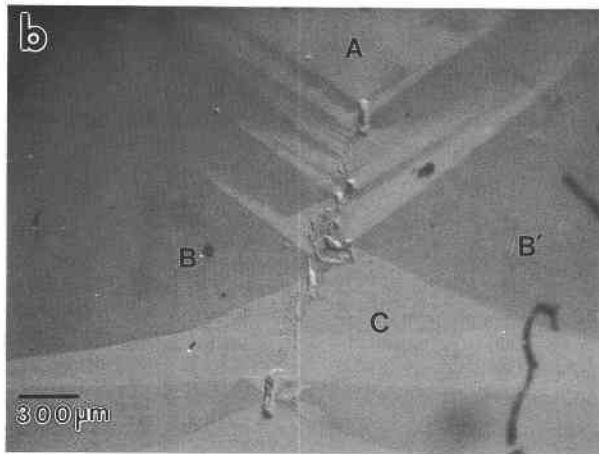
Fig. 3. (a) DIC photomicrograph of a growth hillock on (110) of a second topaz crystal, in the same orientation as Fig. 1. Macrosteps are apparent and show complex growth around an outcropping inclusion. (b) Corresponding CL photomicrograph. Note the strict correspondence of the CL pattern to the complex microtopography and to the mirror symmetry. Observed CL colors are the same as in Fig. 2.
