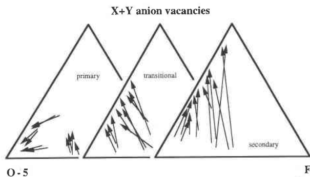
Fig. 4. Triangular plots (atomic percent) of X-site and Y-site anions and X + Y anion vacancies in unaltered and altered pyrochlore samples. The O content is plotted as O – 5 to give the same scale as Fig. 3.
