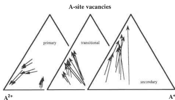
Fig. 3. Triangular plots (atomic percent) of divalent A-site cations (mainly Ca plus some Fe, Sr, and Ba), monovalent A-site cations (mainly Na plus minor K), and A-site vacancies in unaltered and altered pyrochlore samples. Alteration vectors are shown as arrows pointing toward the altered composition.
