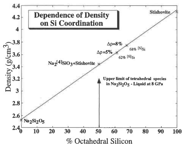
FIGURE 7. Densities of hypothetical assemblages of Na 2 Si 2 O 5 composition as a function of octahedral Si content. The densities of the largely tetrahedral phases were estimated from a linear fit to the densities as a function of composition for seven low-pressure sodium silicate crystalline phases: Na 2 Si 3 O 7 (Williamson and Glasser 1966); Na 6 Si 8 O 19 (Williamson and Glasser 1965); α-Na 2 Si 2 O 5 (Williamson and Glasser 1966); β-Na 2 Si 2 O 5 (Williamson and Glasser 1966); Na 2 SiO 3 (Grund and Pizy 1952); Na 2 Si 2 O 5 (Kautz et al. 1970); and Na 4 SiO 4 (Olazcuaga et al. 1975). We utilize the density of stishovite as a proxy for the density of a phase containing 100% 6 Si. This approximation should yield a lower bound on the change in 6 Si content for a given change in density of an amorphous Na 2 Si 2 O 5 phase. Note that we examine relative changes in density during shifts in coordination, rather than the absolute value of the density produced by different coordination environments.
