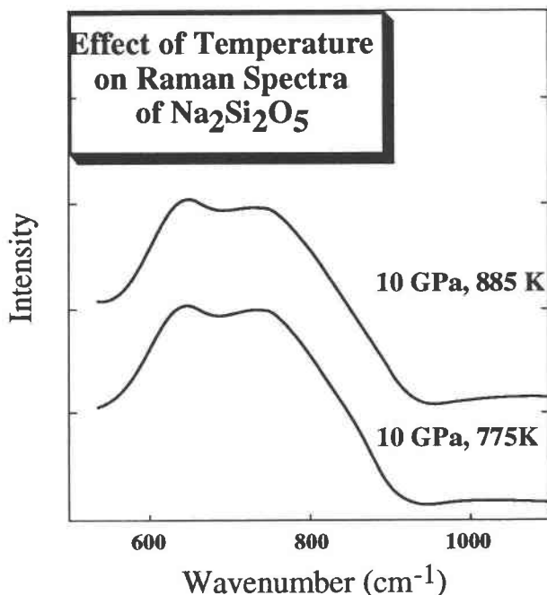
FIGURE 1. Effect of temperature on the Raman spectra of liquid \text{Na}_2\text{Si}_2\text{O}_5 at 10 GPa.
