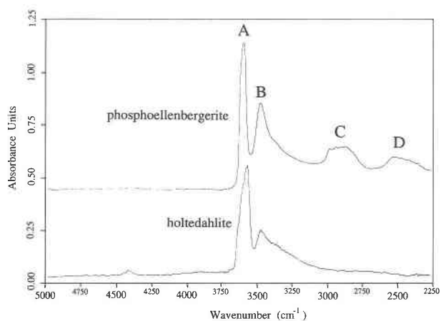
FIGURE 3. Single-crystal IR spectra of phosphoellenbergerite and holtedahllite (100 and 500 scans, respectively). Note that band A is truncated for both phases.
