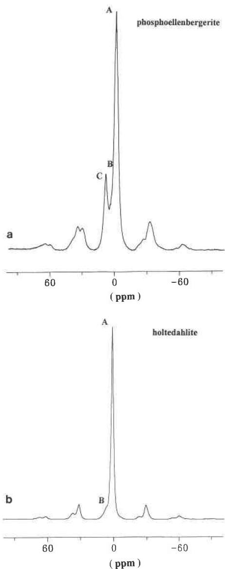
FIGURE 5. The ^1\text{H} MAS NMR spectra of (a) phosphoellenbergerite and (b) holtedahlite recorded at a spinning frequency of 10.0 kHz. Note that only resonances A and B show spinning sidebands.
