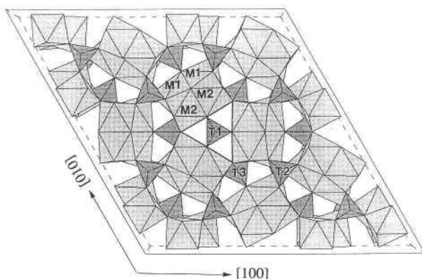
FIGURE 2. View along the c axis of the holtedahllite structure.
