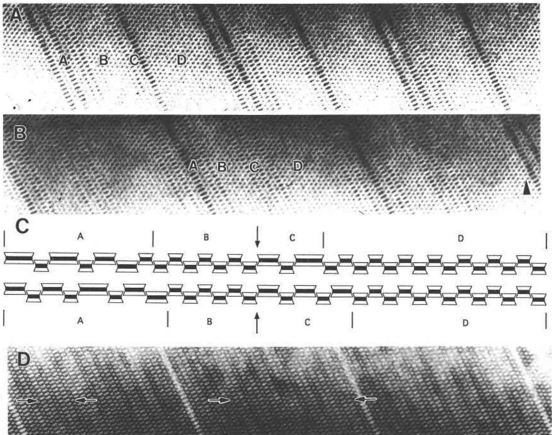
FIGURE 4. Triple repetition of two giant polysomes: (A) 424233(2)^*324(2)^{15} and (B) 32324233(2)^*(32)^3(2)^{12} . The images are printed as negatives to enhance the contrast. The last faulted sequence in B (arrow) is the same as the first faulted sequence in A. (C) I-beam representation of both giant polysomes. A and C indicate the faulted sectors, whereas B and D are the unfaulted
