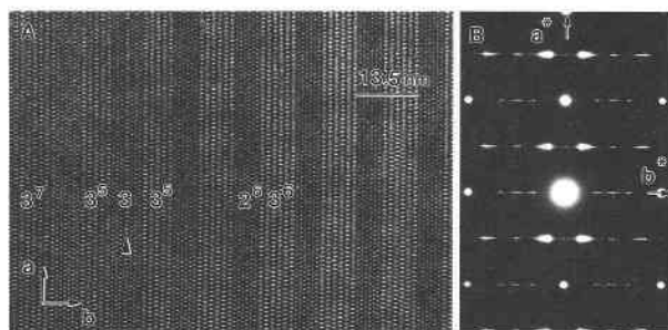
FIGURE 1. (A) The [001] high-resolution electron transmission microscopy (HRTEM) image and (B) selected-area electron diffraction (SAED) pattern of the (2^6 3^6) polysome. The numbers of individual chains in some lamellae are indicated. Chain-width faults, such as the isolated triple-chain slab in a double-chain lamella (arrow), are discussed in the text. All subsequent HRTEM images have the same crystallographic orientation as indicated in Figure 2A, unless otherwise indicated.
