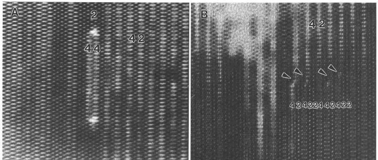
FIGURE 10. (A) A doubly terminated . . . 44 . . . zipper in an anthophyllite lamella near a sequence of the (42) polysome. The widths of the chains at both ends of the zipper cannot be determined with certainty (quintuple or sextuple?). The blurred appearance of the image is due to mechanical drift of the sample
