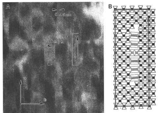
FIGURE 5. (A) HRTEM image of an enstatite grain with a high concentration of isolated amphibole zippers. The different contrast on opposite sides of the zippers is due to different strain. Dark areas are under compression, whereas light areas are dilated. The Burgers circuit (arrowed line) around an amphibole zipper indicates that an extra (010) layer of pyroxene I beams (0.91 nm) is introduced on the left side of the zipper. (B) I-beam model of an incoherent, short amphibole zipper in enstatite. The Burgers circuit is shown as a stippled line.
