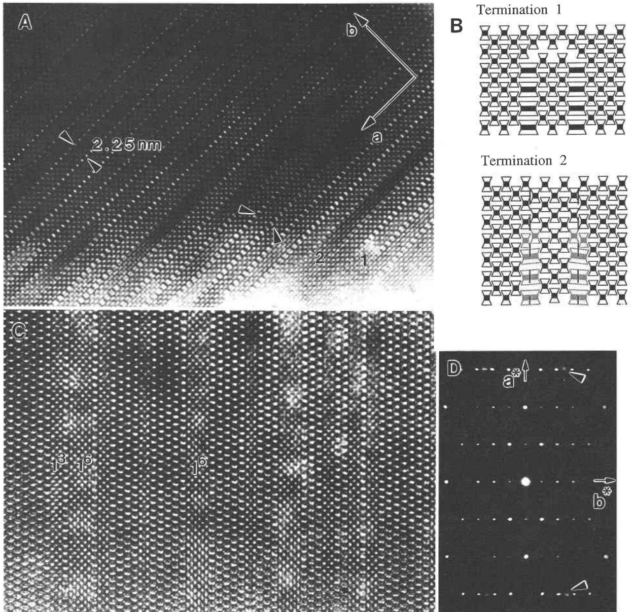
FIGURE 6. (A) HRTEM image of the polysome (2111). Between the arrows the amphibole chains are rotated and the sense of rotation changes from one zipper to the other. The numbers indicate zipper terminations schematically shown in B. (B) 1-beam models of the terminations: 1 = termination created by a cooperative zipper transformation mechanism; 2 = termination created by the simultaneous propagation of two partial dislocations. (C) Amphibole-pyroxene intergrowth. The pyroxene chains
