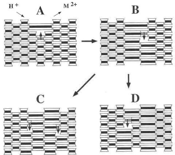
FIGURE 9. Schematic representation of the transformation of double chains into triple chains and ordered (42) sequences: (A) ... 222 ... → ... 6 ...; (B) ... 62 ... → ... 44 ...; (C) ... 2442 ... → ... 2424 ...; (D) ... 2442 ... → ... 3333 ... The arrows show the net displacement of I beams or part of them. Reaction A requires the removal of octahedral cations and the addition of H + whereas all other reaction steps are isochemical.
