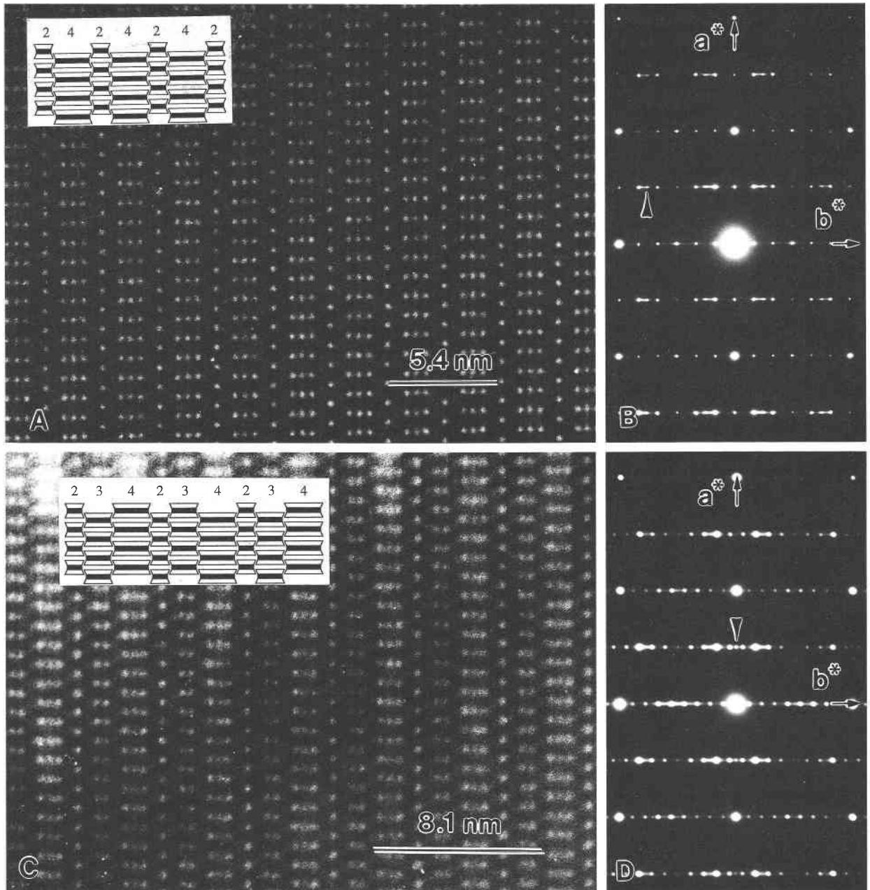
FIGURE 2. HRTEM images and SAED patterns of the [001] zone of the polysome (42) (A and B) and the polysome (234) (C and D). The insets in the images are I-beam representations of the polysomes with the numbers of subchains in each Si tetrahedral chain indicated on top. The arrows in B and D point to diffraction spots belonging to anthophyllite.
