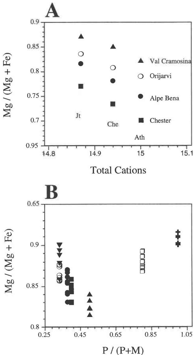
FIGURE 8. (A) Mg/(Mg + Fe) vs. total cations on the M sites of the ordered biopyrribbles from Chester (Veblen and Burnham 1978a), Orijärvi (Schumacher and Czank 1987), Alpe Bena and Val Cramosina. (B) Mg/(Mg + Fe) vs. module composition of some short-range polysomes from Alpe Bena and Val Cramosina: triangles = anthophyllite, open circles = jimthompsonite, solid squares = chesterite, inverted triangles = (42), solid circles = (423232), open squares = enstatite, and plus signs = (2111).
