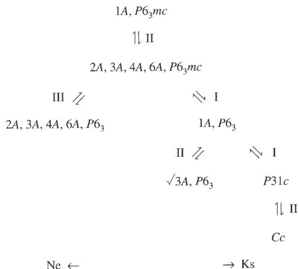
FIGURE 18. Schematic summary of isochemical transitions. Those on the right occur at more Ks-rich compositions, and those on the left at more Ne-rich compositions. Each transition is labeled: I = first-order character because the space groups do not have a supergroup \rightarrow subgroup relationship; II = first-order character because third-order invariants of the order parameter are permitted in the excess free energy; III = thermodynamically continuous character permitted by symmetry.
