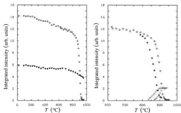
FIGURE 7. (left) Integrated intensities of the 111 (open circles) and 112 (solid triangles) reflections during heating of homogenized Ks_{88} . (right) Integrated intensities of 111 reflection on heating (open circles) and cooling (solid circles), and of the superstructure reflection 12.10 for a cell with a = 4.4 , c = C , on heating (plus signs) and cooling (Xs).
