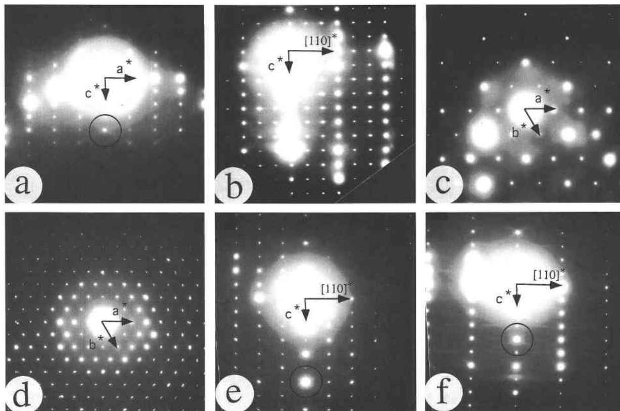
FIGURE 11. Selected-area diffraction patterns, overexposed to reveal diffuse intensity. (a) a^*-c^* section of Ks_{100} . Note the curved bands of diffuse intensity passing through many of the reflections. (b) c^*-[110]^* , kalsilite from Mount Nyiragongo, 75422. Superstructure reflections defining tripling parallel to [110]^* are diffuse. Some weak, curved diffuse bands similar to those in a were more clearly visible on the original photographic plate. (c) a^*-b^* , kalsilite from Mount Nyiragongo, 75422. The \sqrt{3}A superstructure reflections are highly diffuse in this case. (d) a^*-b^* , exsolved nepheline from Alban Hills. The smearing of individ-
