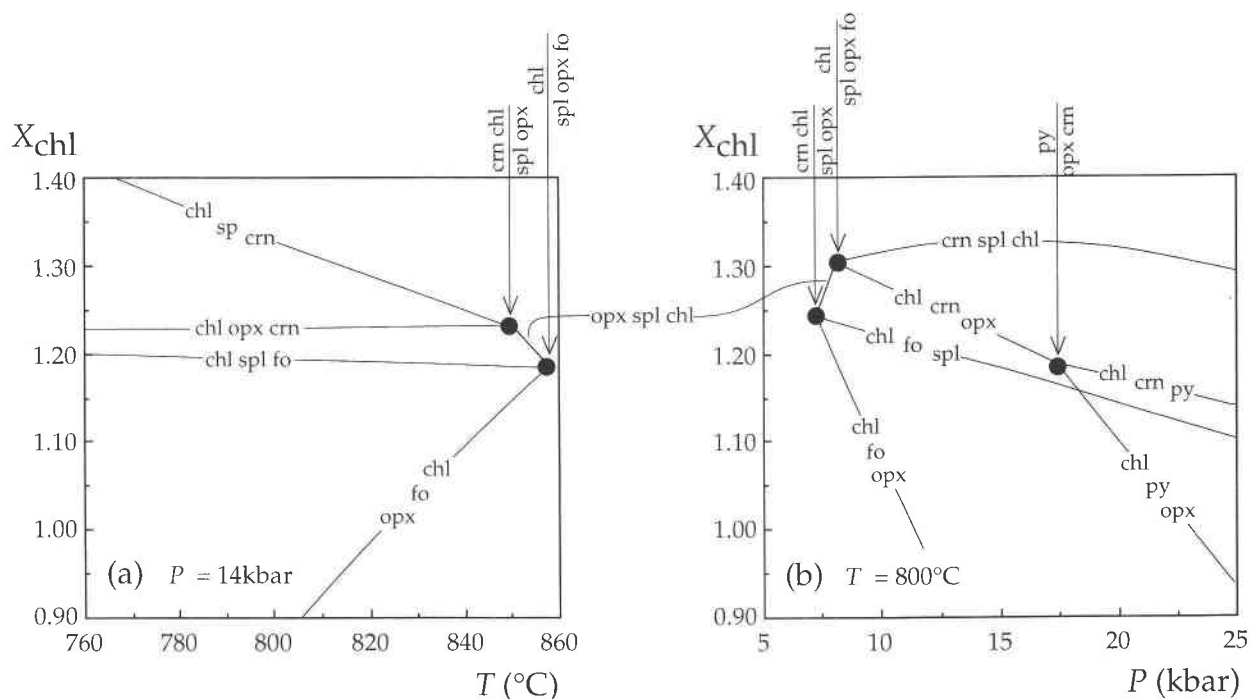
FIGURE 3. The variation of X_{chl} in divariant assemblages at (a) P = 14 kbar and (b) T = 800 °C, calculated using the simple a - X model of Holland and Powell (1990). Mineral abbreviations as in Figure 1. Solid circles show the conditions at which univariant reactions take place; the reaction taking place in each case is given on the adjacent arrow.
