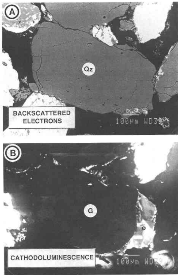
FIGURE 4. SEM photomicrograph of quartz from a Keuper sandstone from borehole B3. (A) Backscattered electron image showing the dark gray quartz (Qz) and (B) CL image of the same quartz showing the dark luminescent detrital grain (G) and the bright luminescent overgrowth (o); note the bright patterns in the overgrowth.
