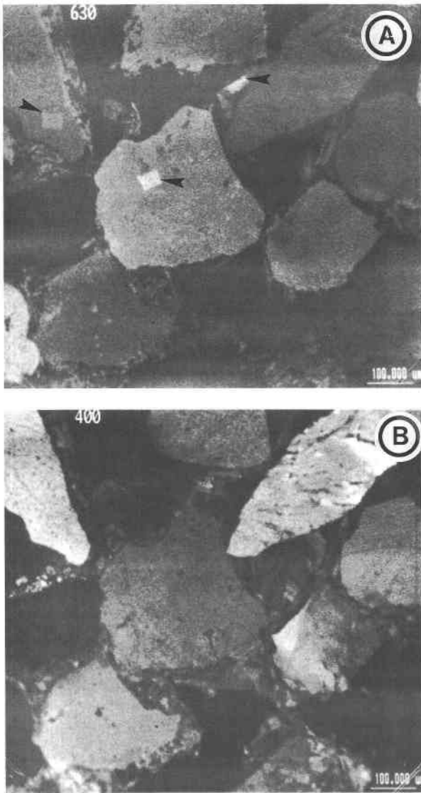
FIGURE 7. SEM photomicrograph of cathodoluminescence at various wavelengths. (A) At 630 nm, arrows show the location of prolonged electron bombardment. Note the higher cathodoluminescence signal of these areas. (B) At 400 nm, bombarded areas do not show any variation of the cathodoluminescence signal.
