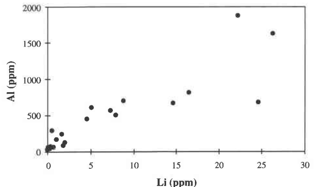
FIGURE 9. Plot of Al vs. Li contents of quartz determined by ion probe.
