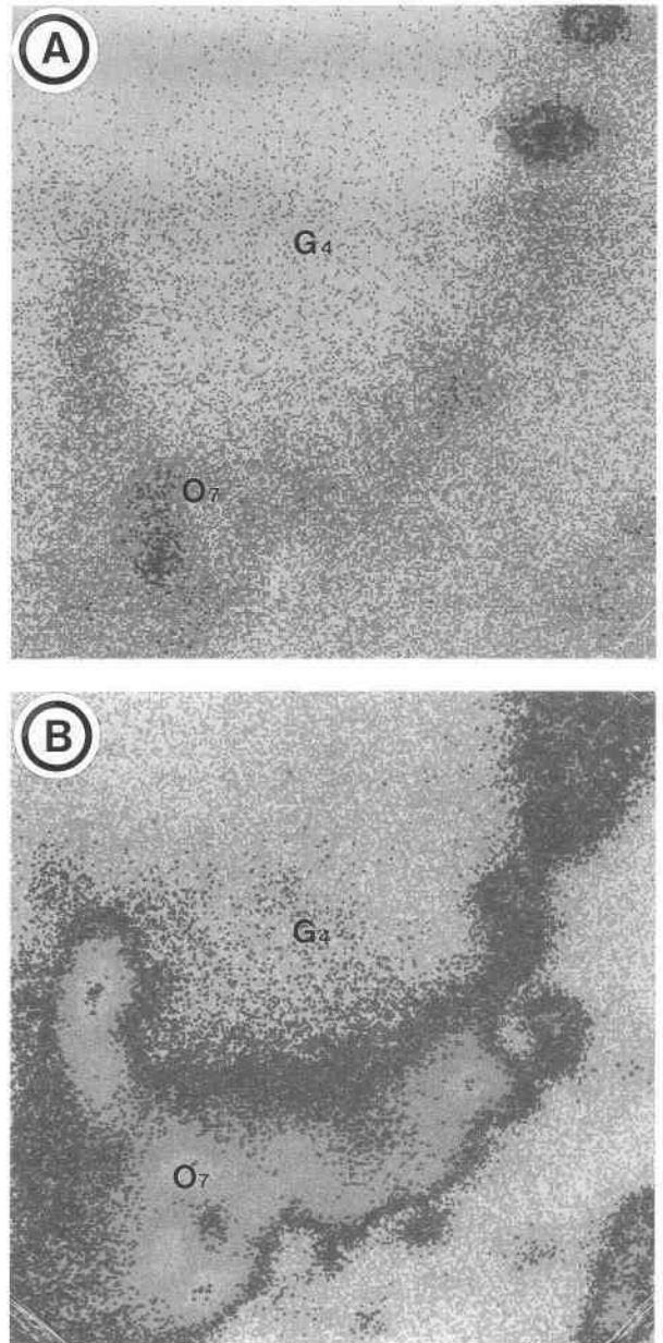
FIGURE 11. Ionic images of the area shown in Figure 5, including quartz grain G4 and overgrowth O7. (A) Li image: The highest signal is shown in the overgrowth O7 (black); (B) Al image: The highest signal is shown in the overgrowth O7 (dark gray). The ionic images are inverted in comparison with standard SEM photomicrographs.
